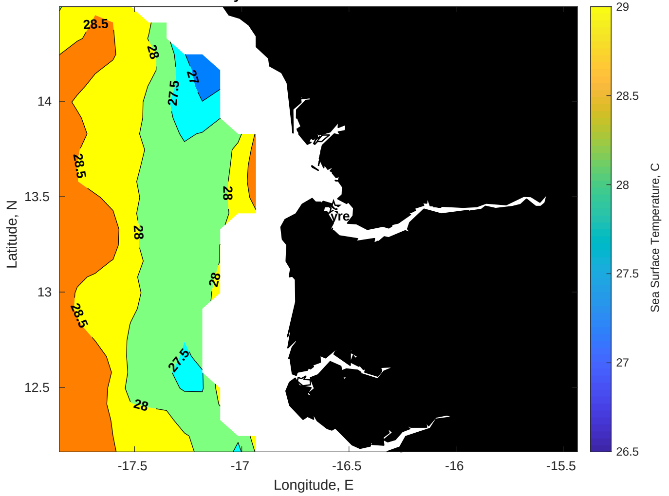
SST for Gyre at 29-Jun-2025 00:00:00
