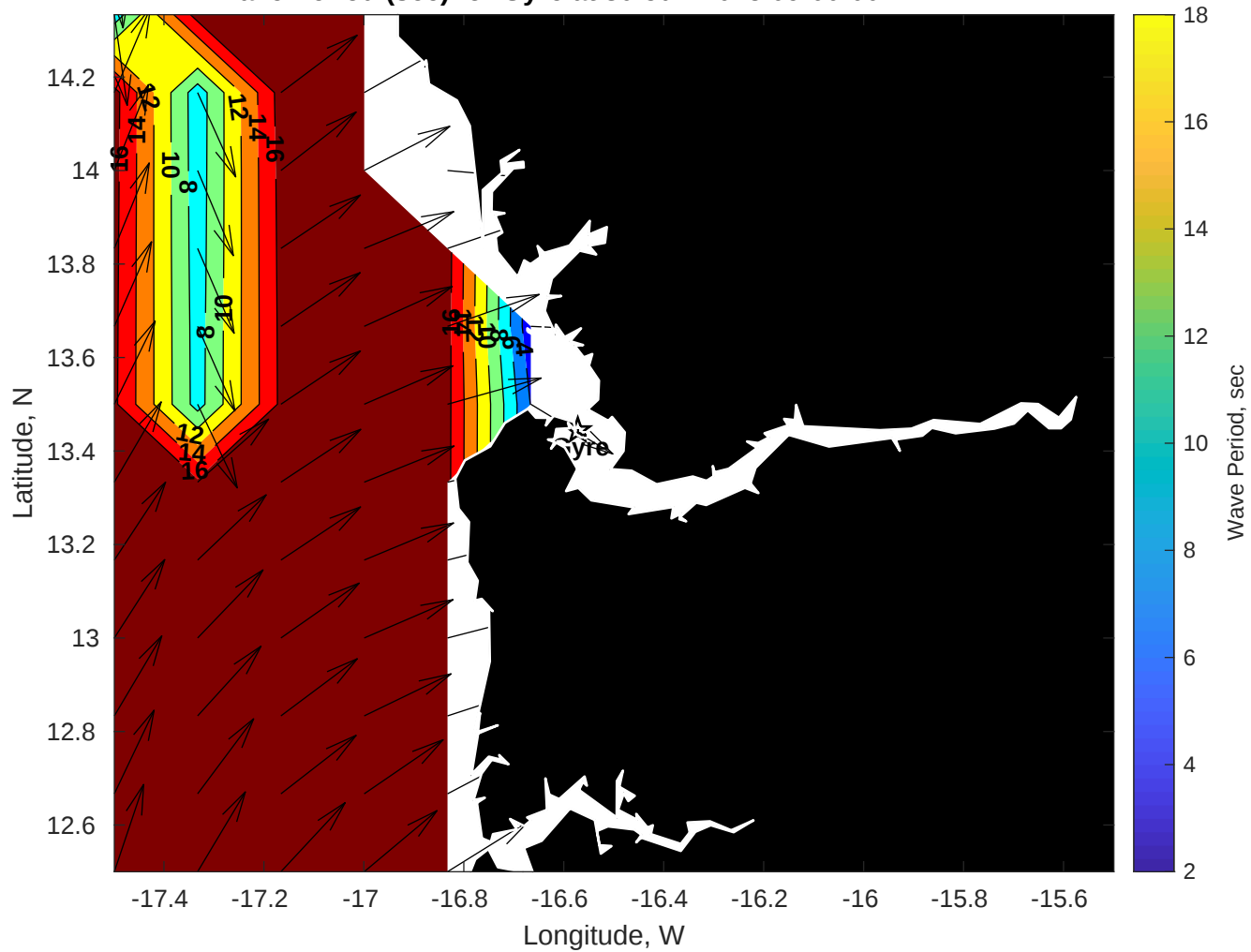
Wave Period (sec) for Gyre at 30-Jun-2025 09:00:00
