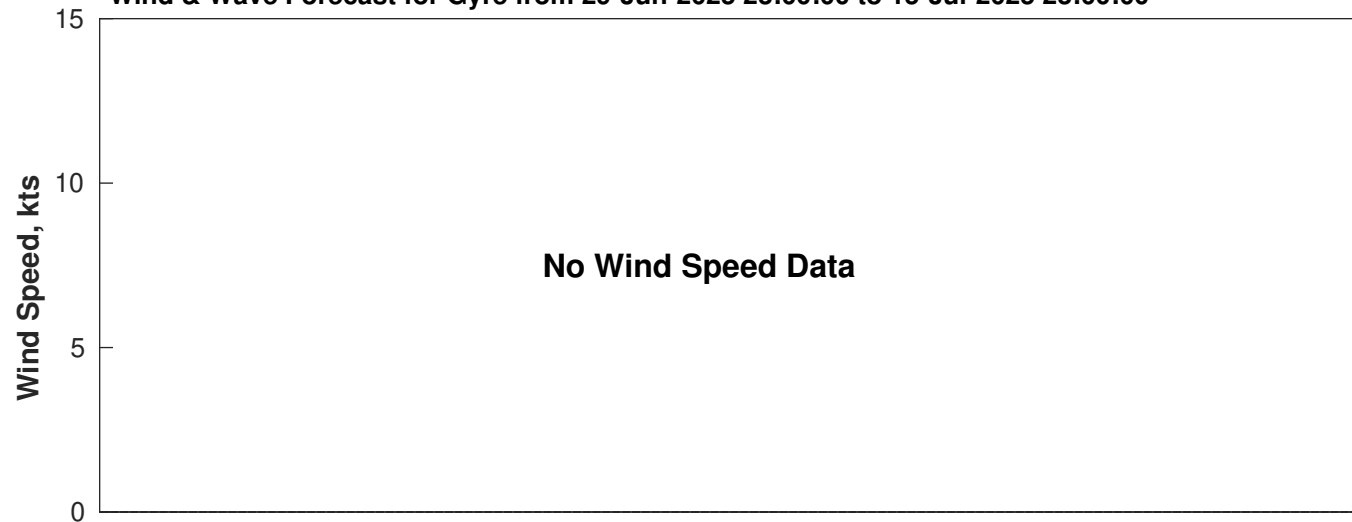
Wind & Wave Forecast for Gyre from 29-Jun-2025 23:00:00 to 15-Jul-2025 23:00:00
