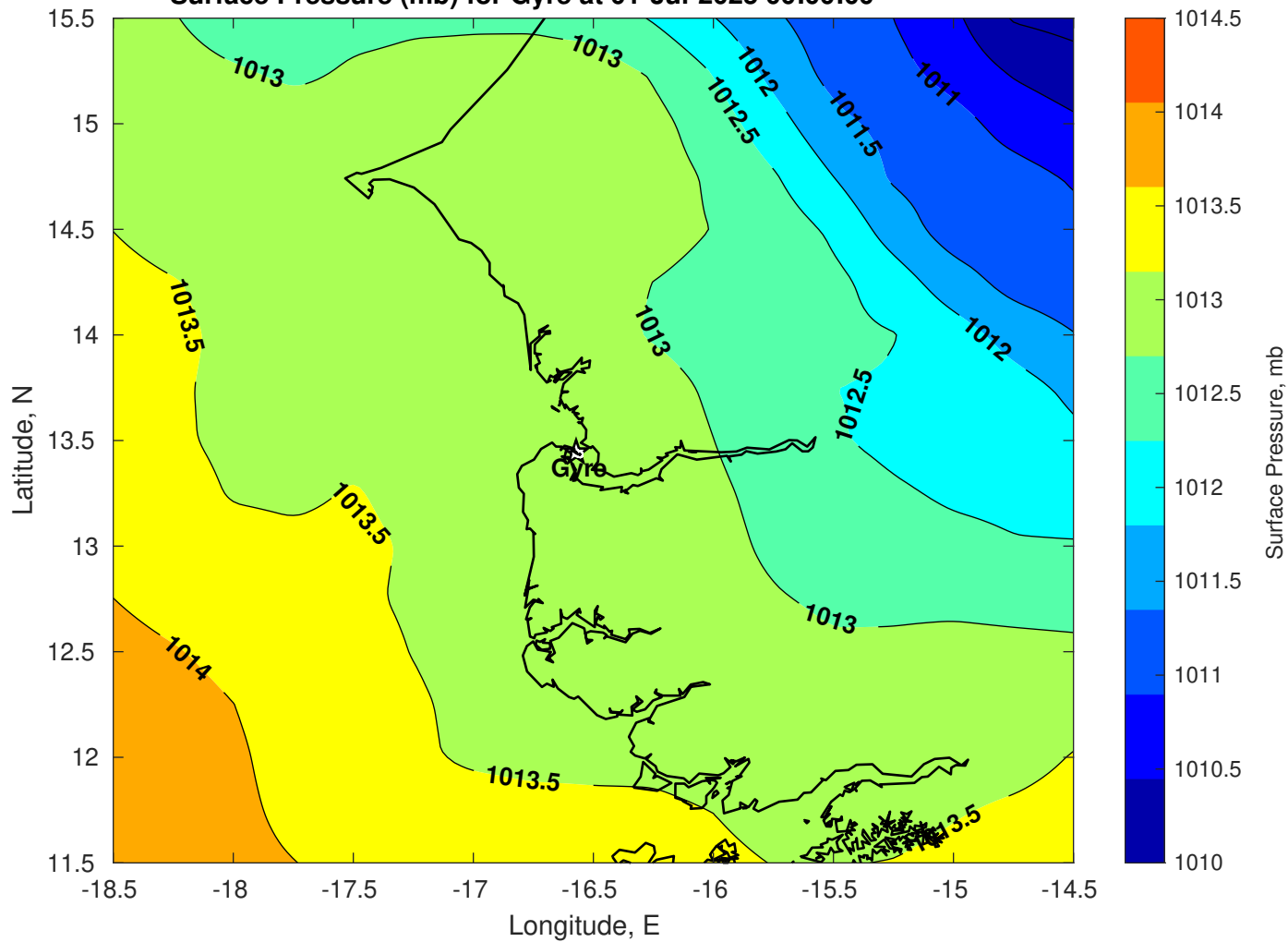
Surface Pressure (mb) for Gyre at 01-Jul-2025 00:00:00
