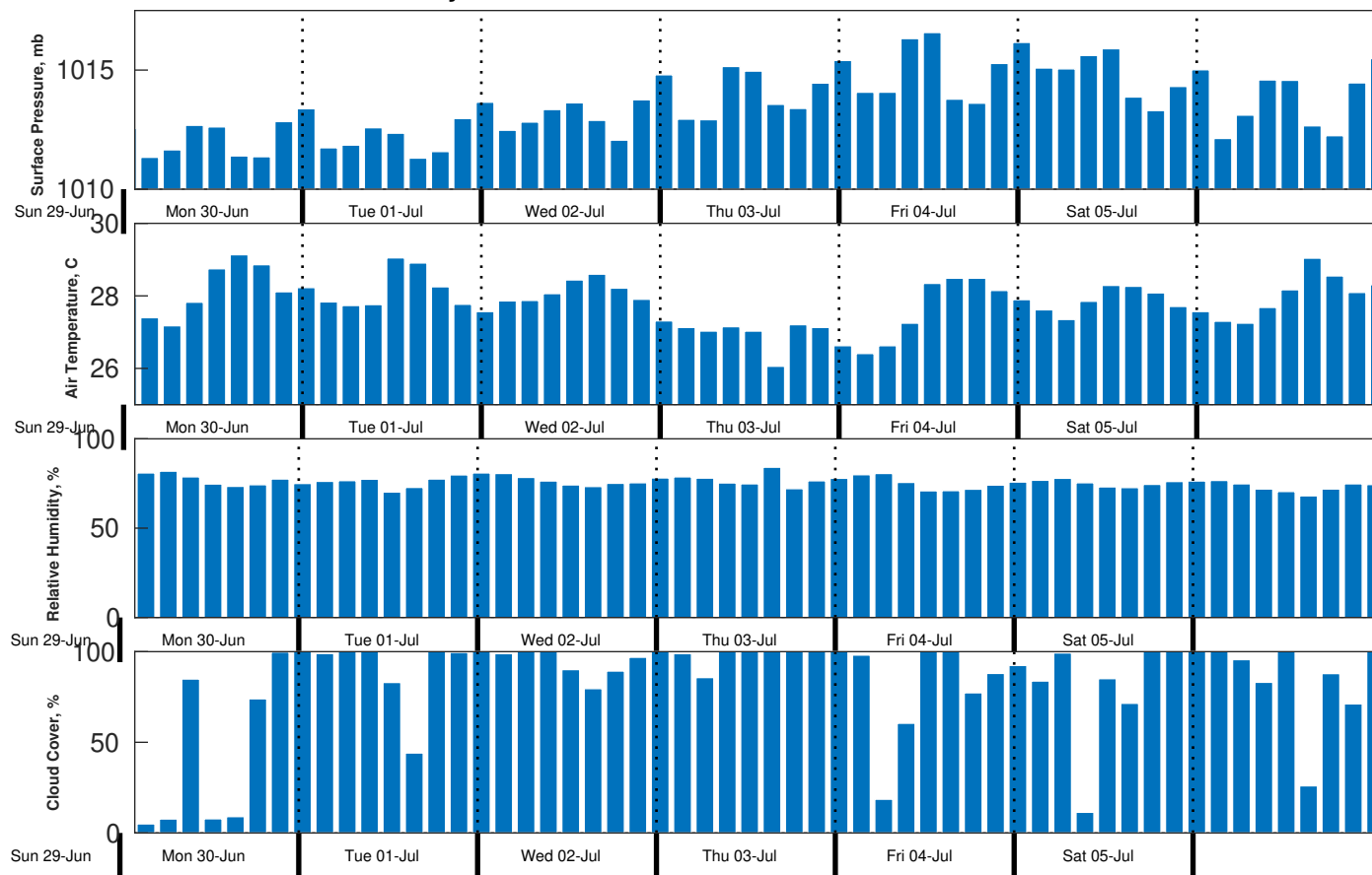
Met Forecast for Gyre from 29-Jun-2025 23:00:00 to 06-Jul-2025 23:00:00
