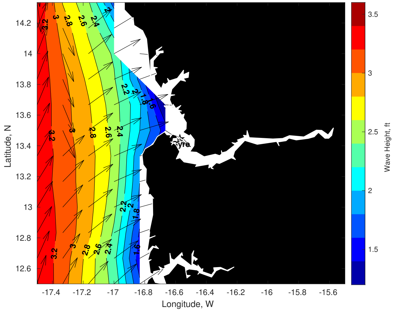
Wave Height (ft) for Gyre at 30-Jun-2025 09:00:00
