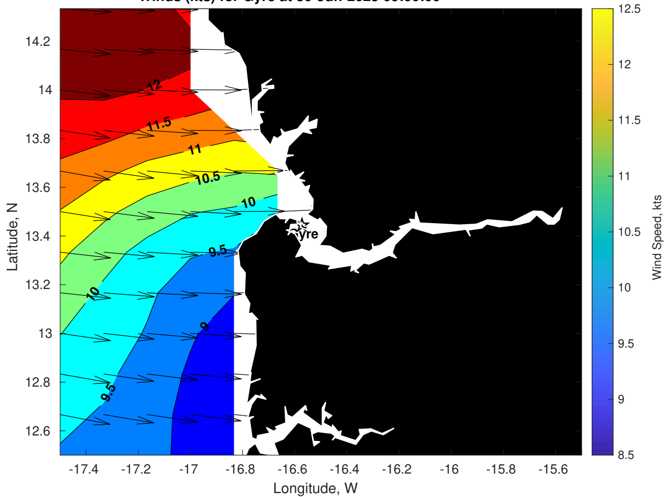
Winds (kts) for Gyre at 30-Jun-2025 09:00:00
