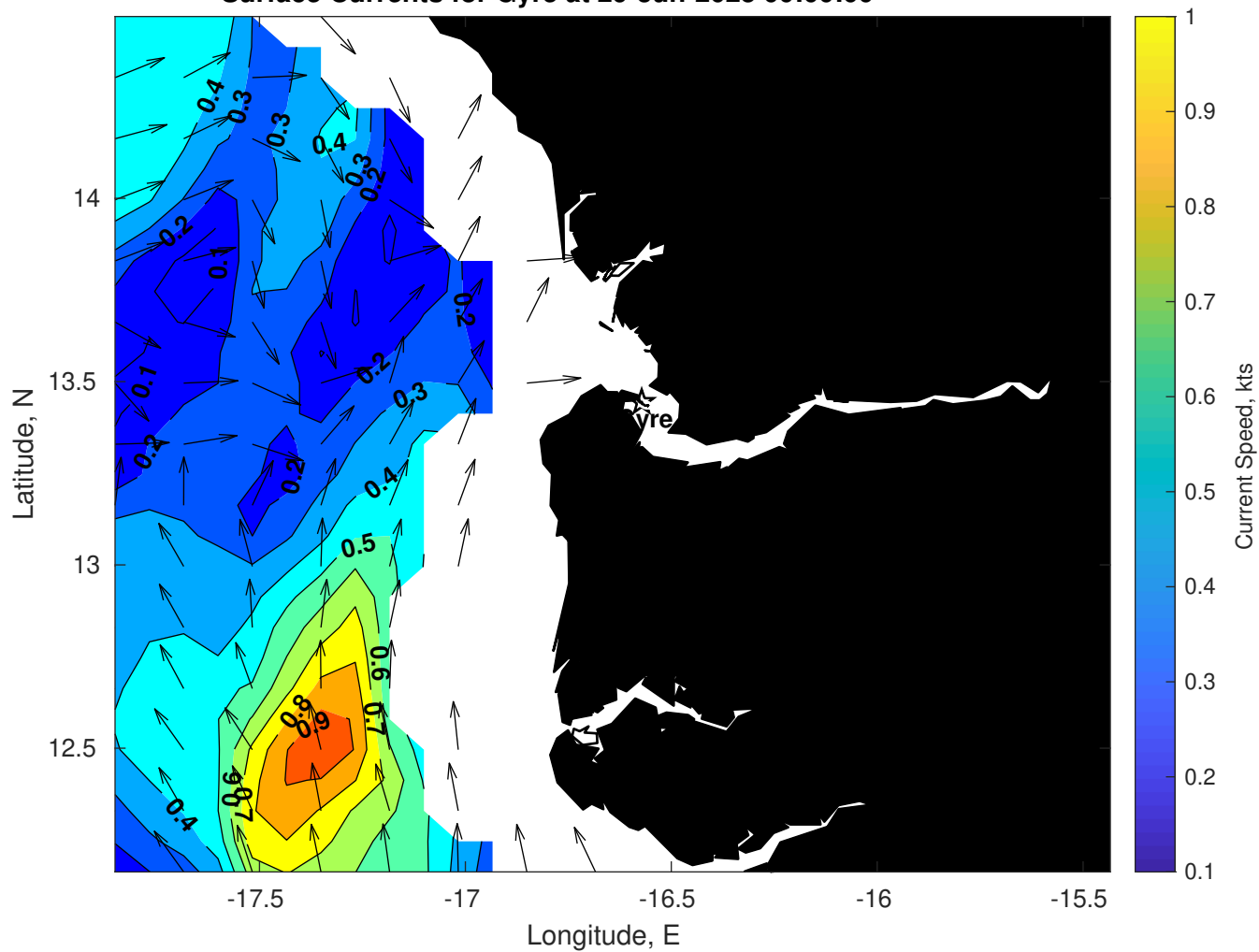
Surface Currents for Gyre at 29-Jun-2025 00:00:00
