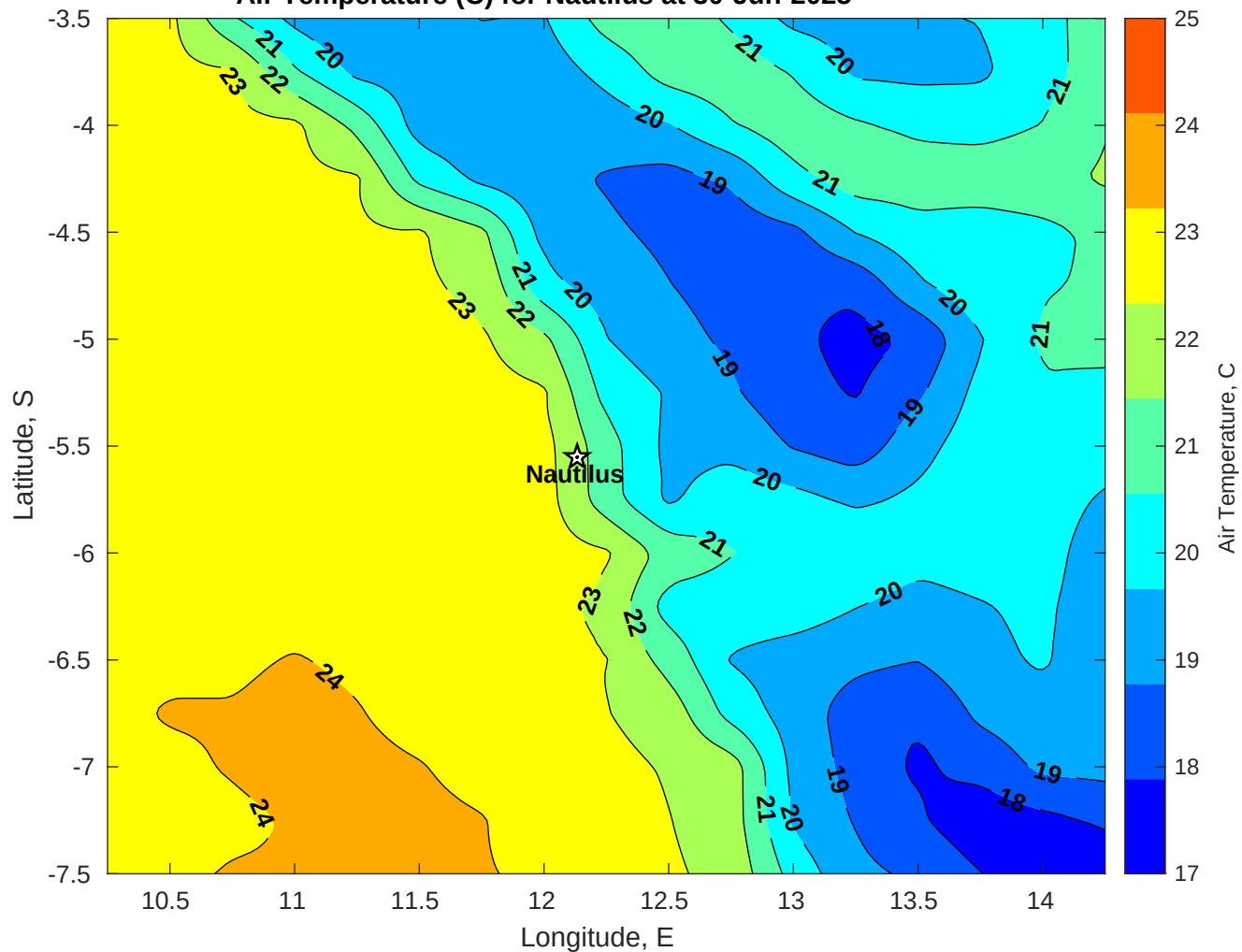
Air Temperature (C) for Nautilus at 30-Jun-2025
