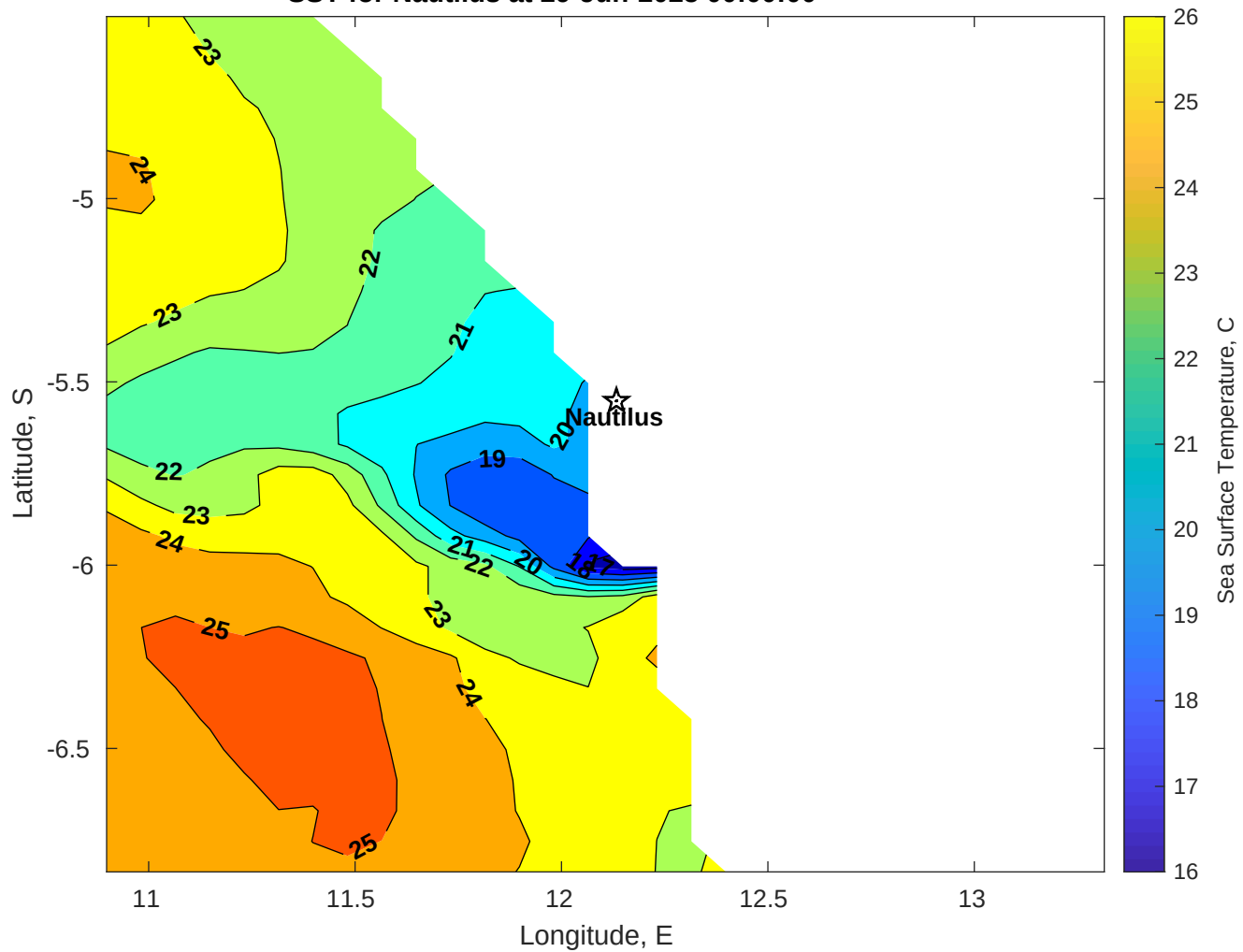
SST for Nautilus at 29-Jun-2025 00:00:00
