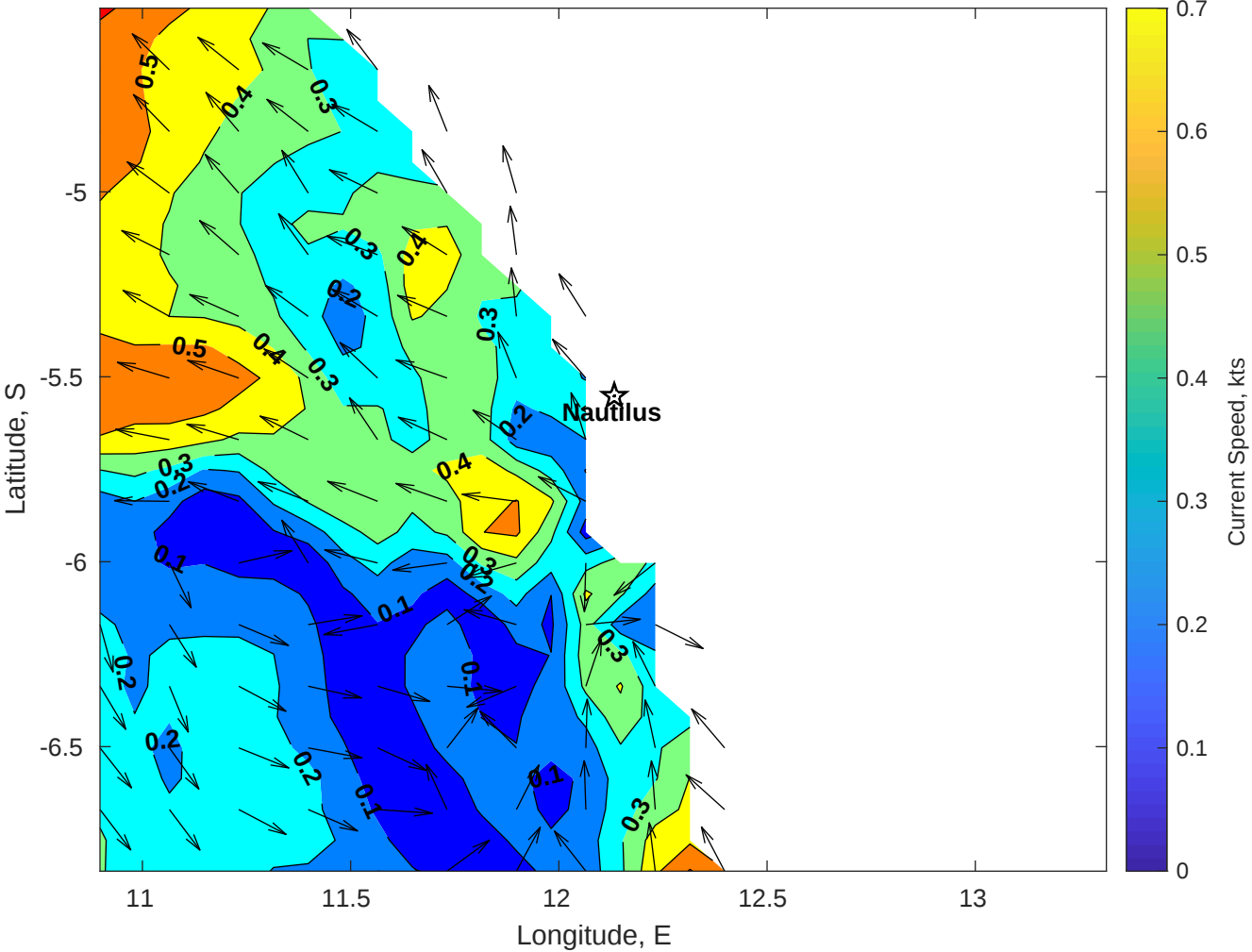
Surface Currents for Nautilus at 29-Jun-2025 00:00:00
