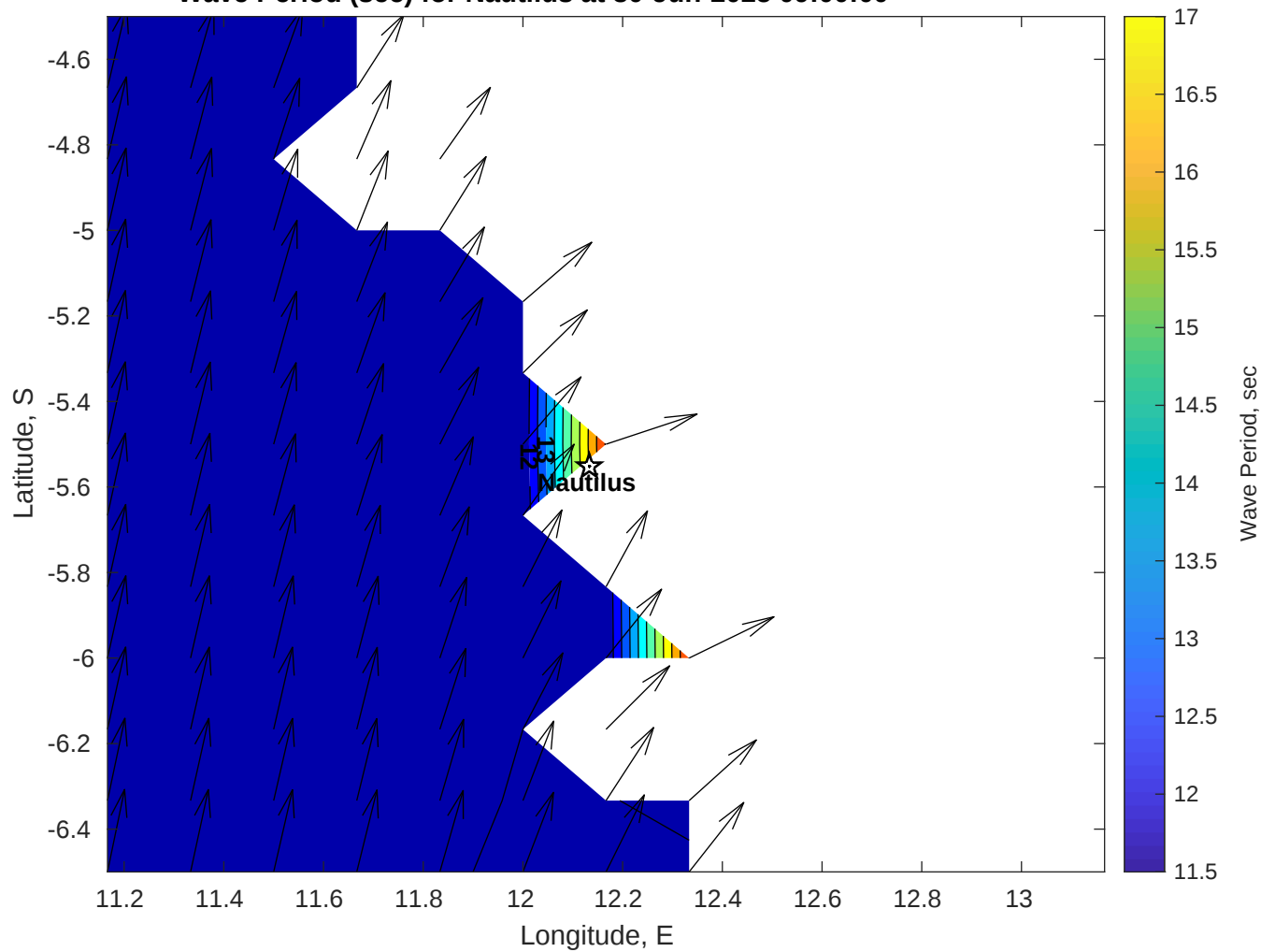
Wave Period (sec) for Nautilus at 30-Jun-2025 09:00:00
