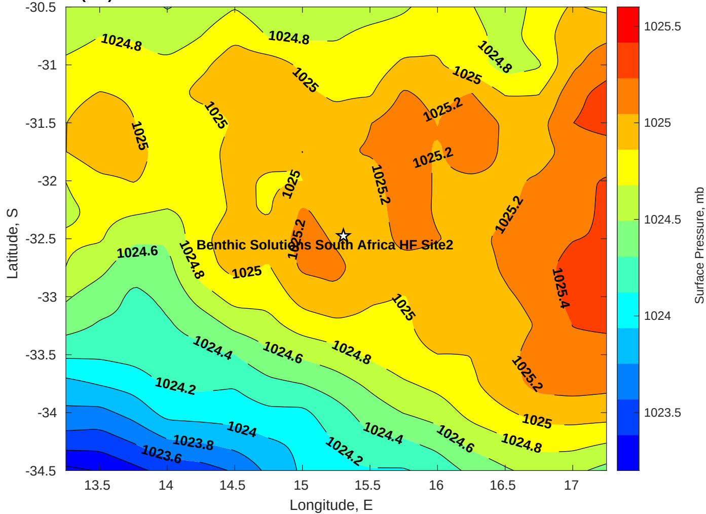
Surface Pressure (mb) for Benthic Solutions South Africa HF Site2 at 21-Jun-2025 00:00:00
