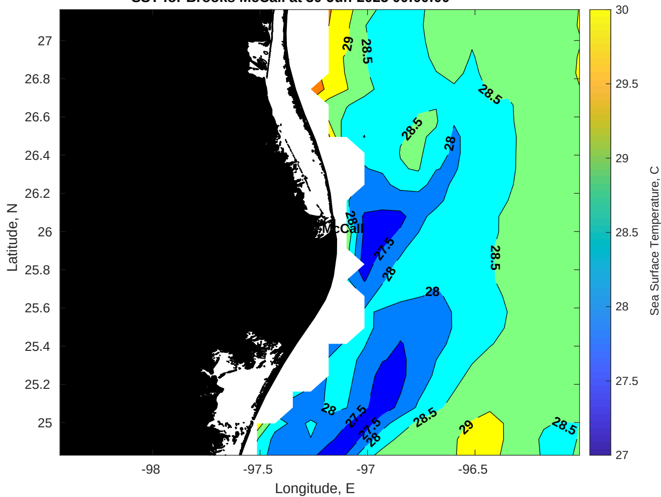
SST for Brooks McCall at 30-Jun-2025 00:00:00
