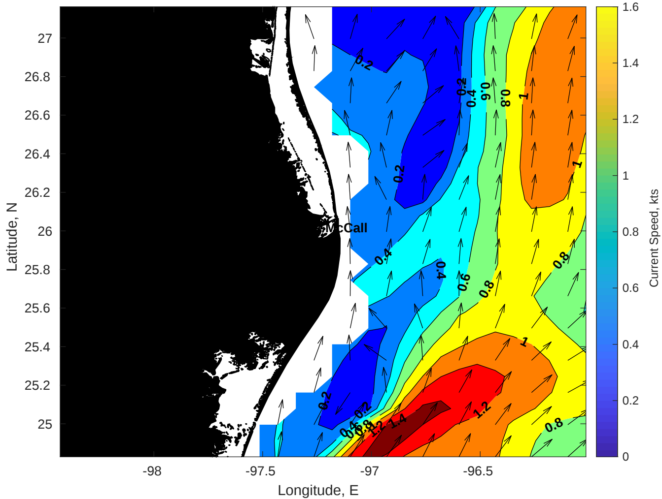
Surface Currents for Brooks McCall at 30-Jun-2025 00:00:00
