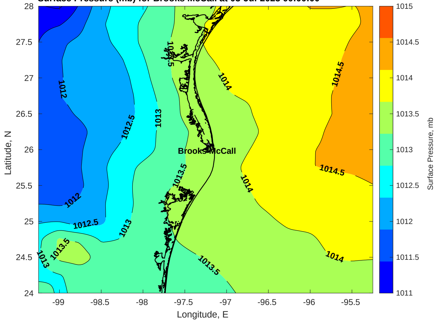
Surface Pressure (mb) for Brooks McCall at 03-Jul-2025 00:00:00
