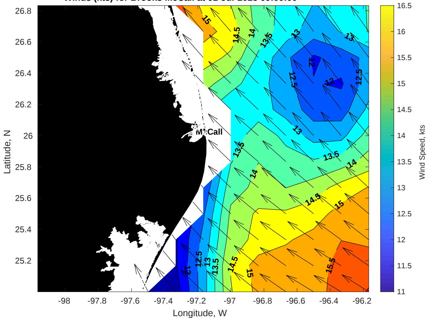
Winds (kts) for Brooks McCall at 01-Jul-2025 09:00:00
