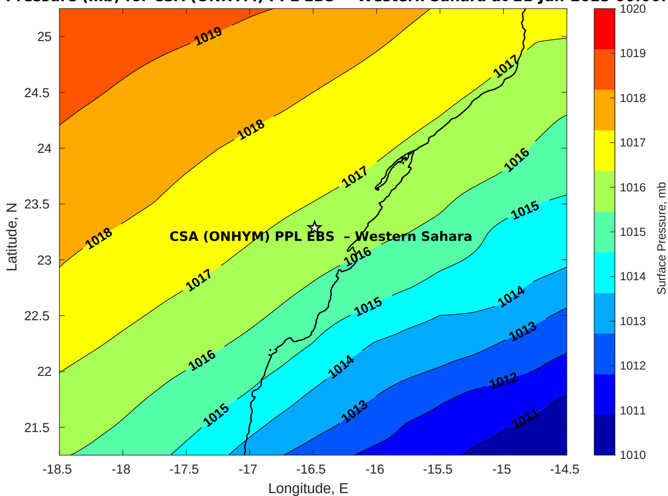
Surface Pressure (mb) for CSA (ONHYM) PPL EBS - Western Sahara at 21-Jun-2025 00:00:00
