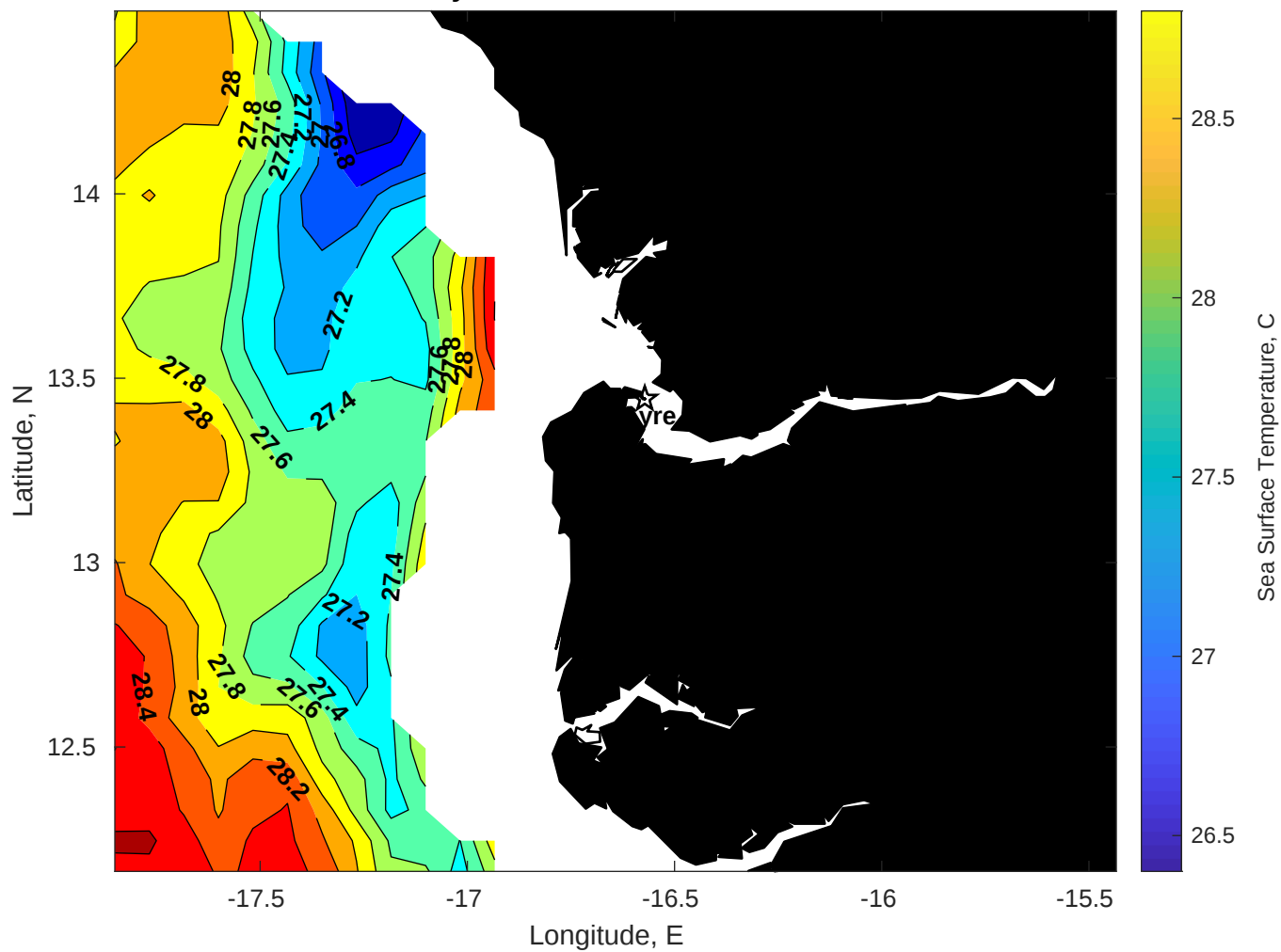
SST for Gyre at 30-Jun-2025 00:00:00
