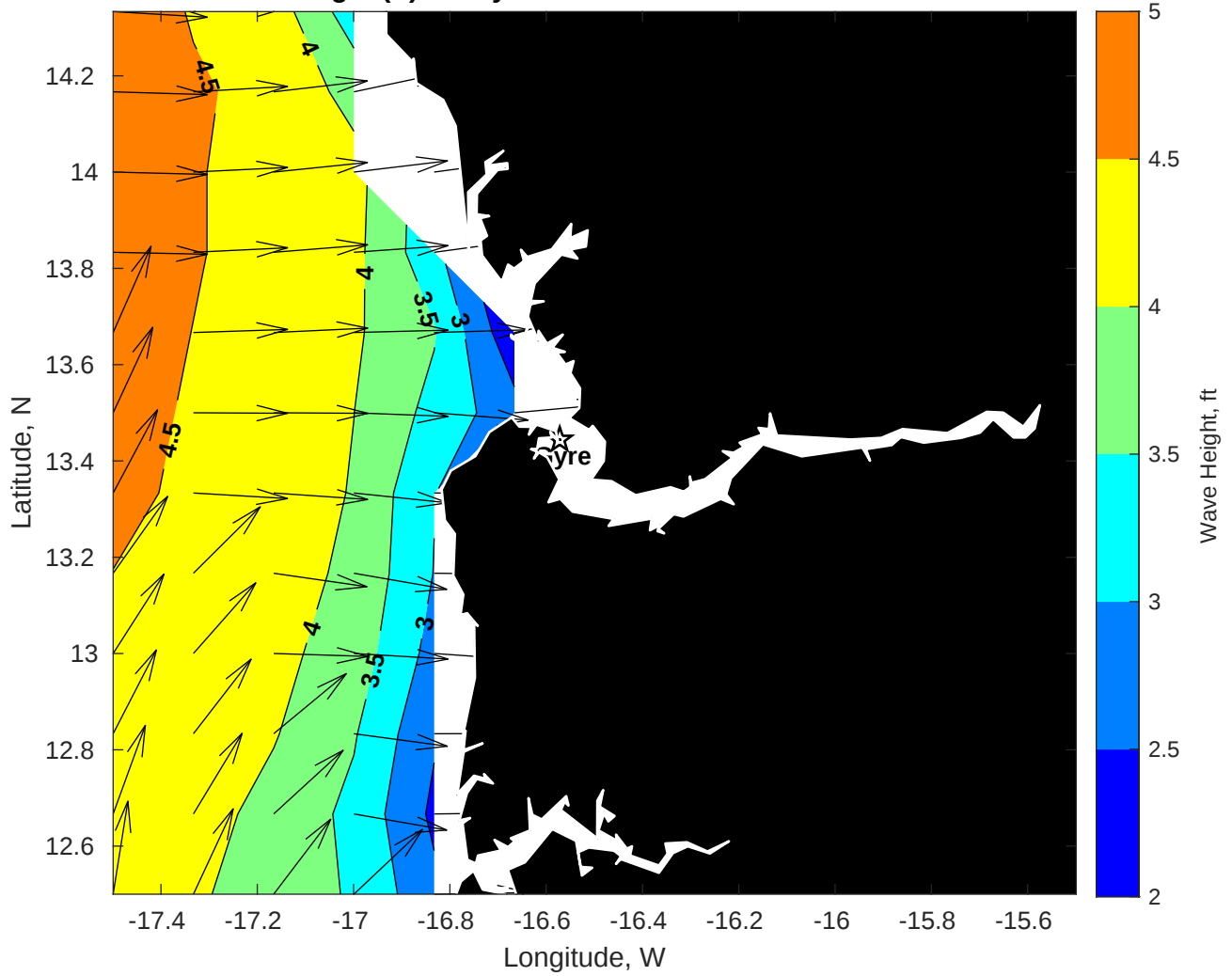
Wave Height (ft) for Gyre at 01-Jul-2025 09:00:00
