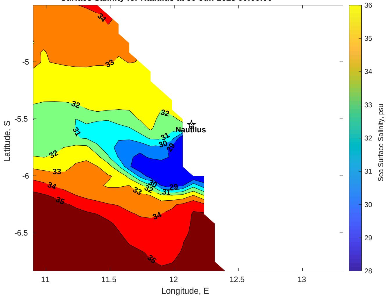
Surface Salinity for Nautilus at 30-Jun-2025 00:00:00
