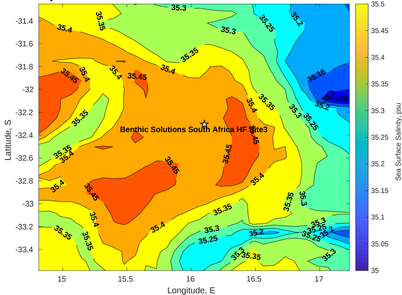
Surface Salinity for Benthic Solutions South Africa HF Site3 at 07-Jun-2025 00:00:00
