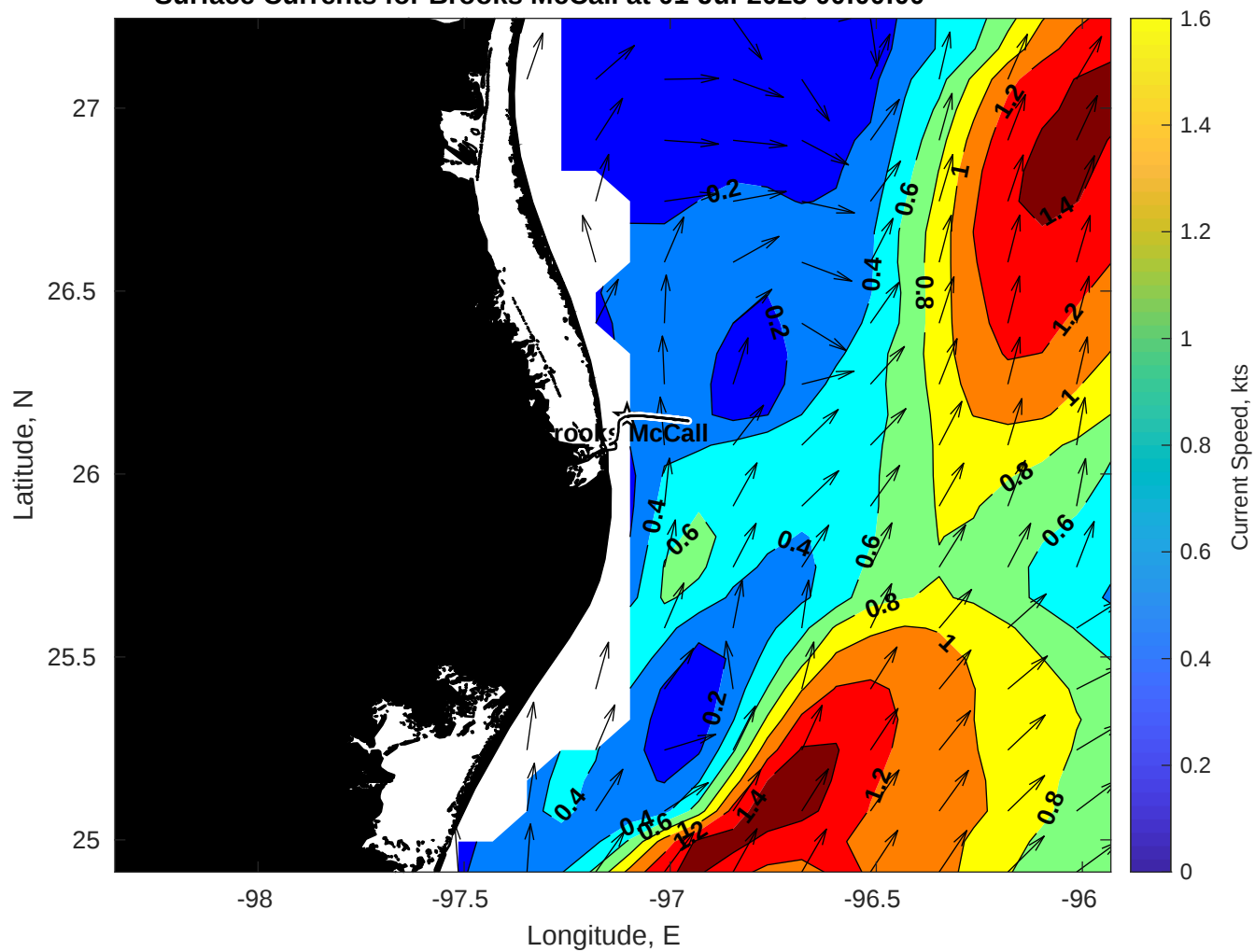
Surface Currents for Brooks McCall at 01-Jul-2025 00:00:00
