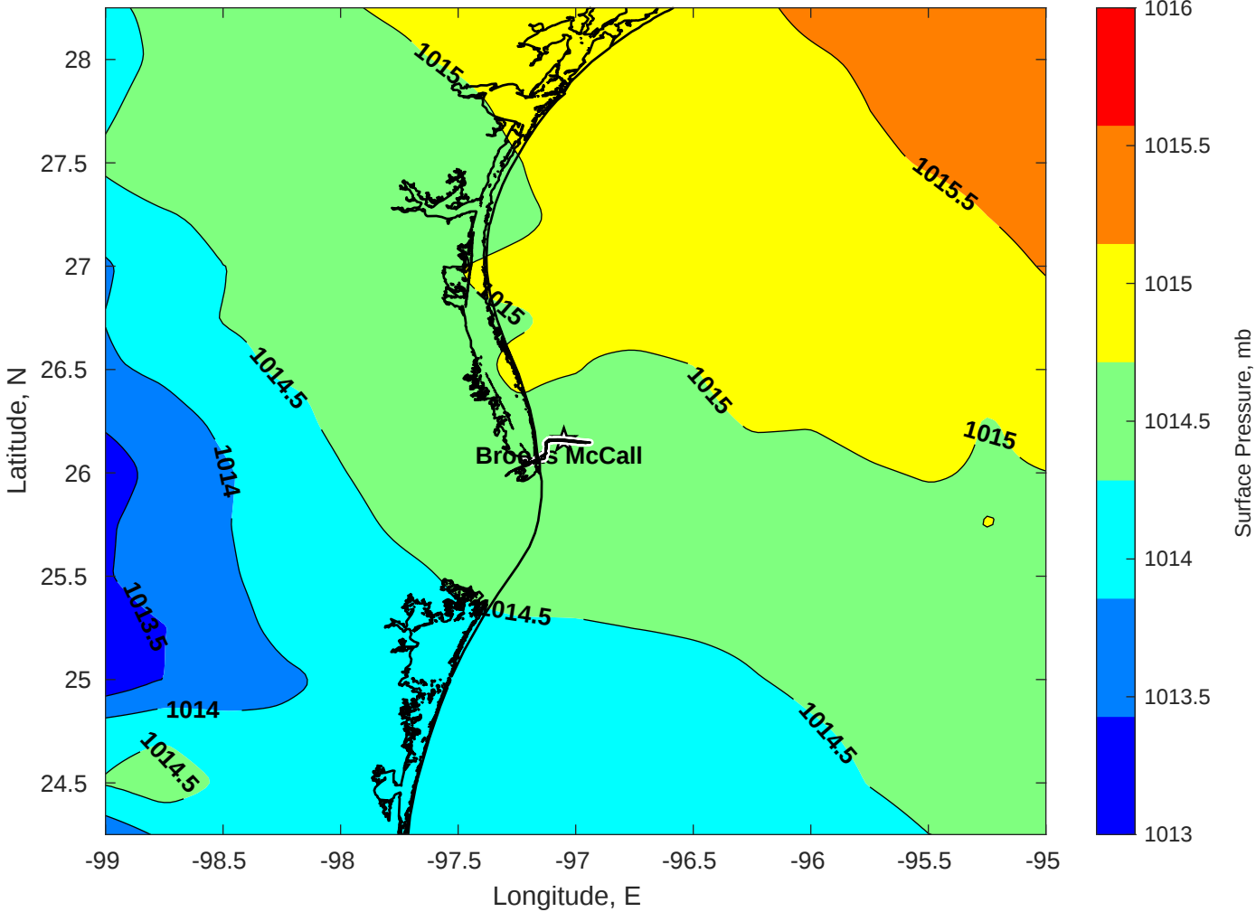
Surface Pressure (mb) for Brooks McCall at 02-Jul-2025 00:00:00
