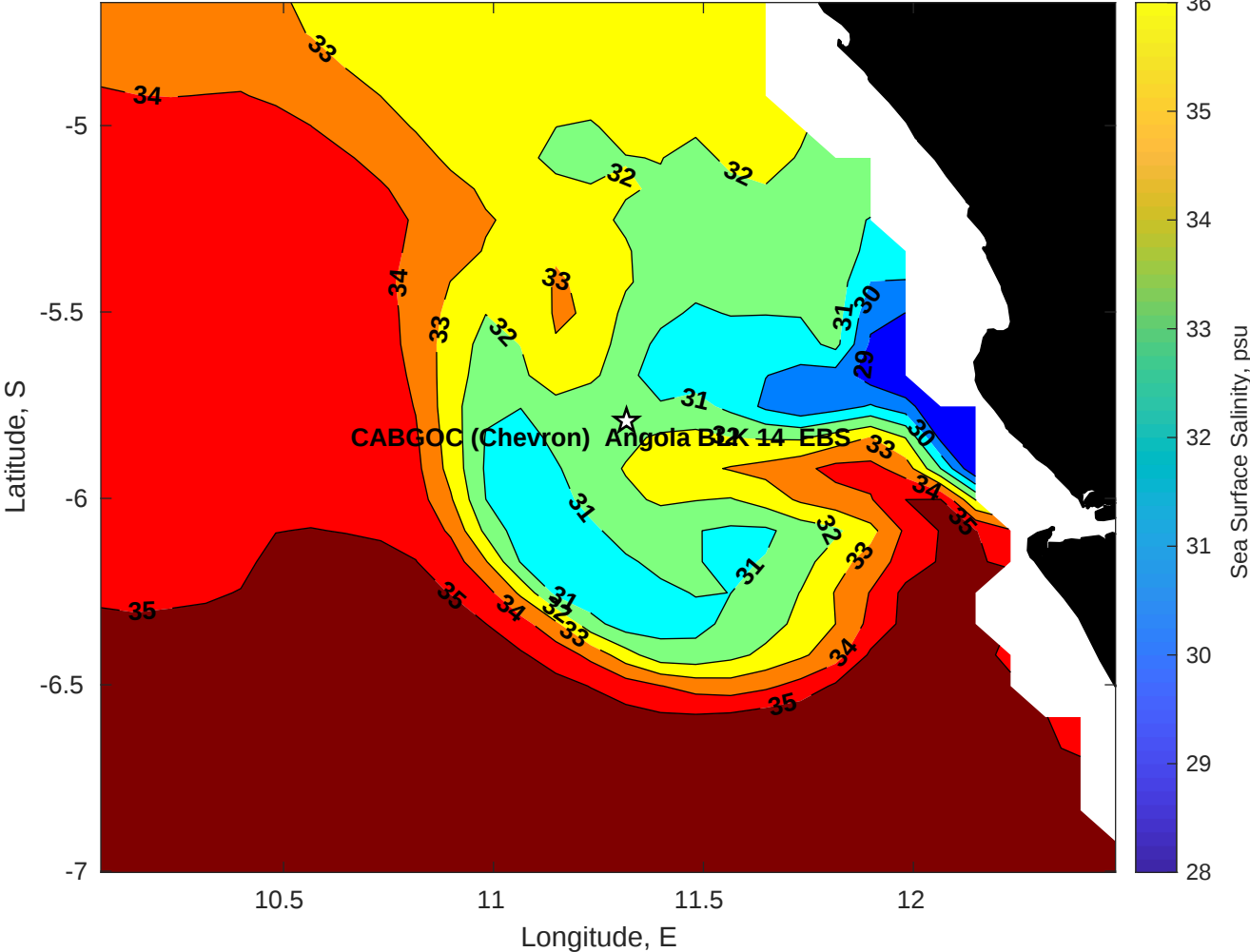
Surface Salinity for CABGOC (Chevron) Angola BLK 14 EBS at 07-Jun-2025 00:00:00
