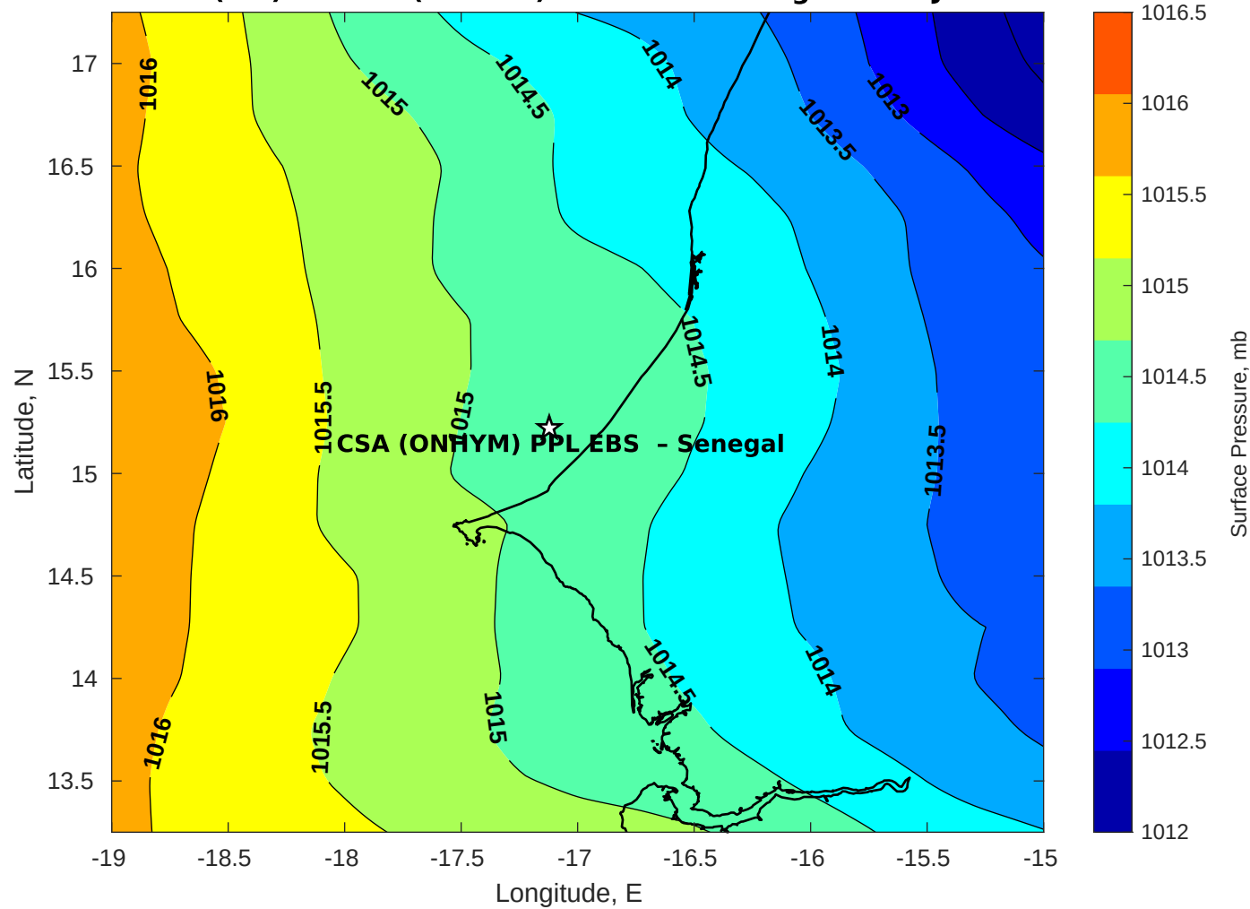
Surface Pressure (mb) for CSA (ONHYM) PPL EBS - Senegal at 19-Jun-2025 00:00:00
