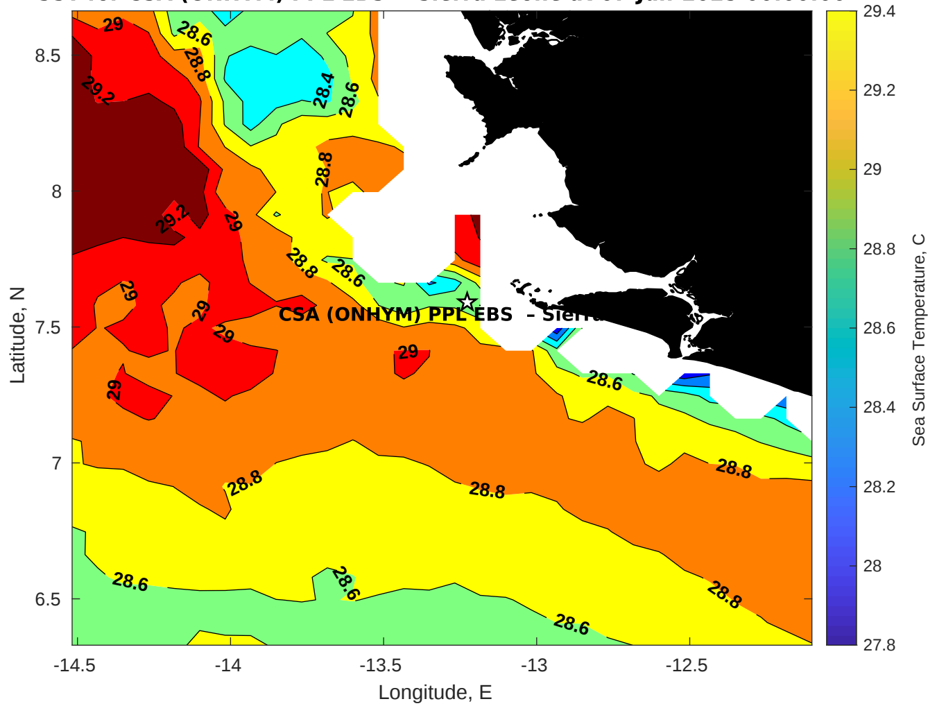
SST for CSA (ONHYM) PPL EBS - Sierra Leone at 07-Jun-2025 00:00:00
