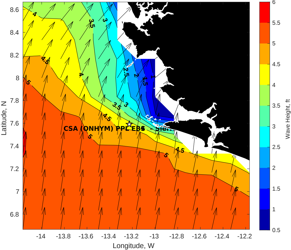
Wave Height (ft) for CSA (ONHYM) PPL EBS - Sierra Leone at 19-Jun-2025 09:00:00
