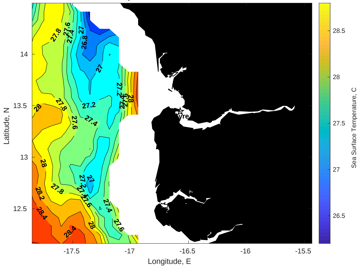
SST for Gyre at 01-Jul-2025 00:00:00
