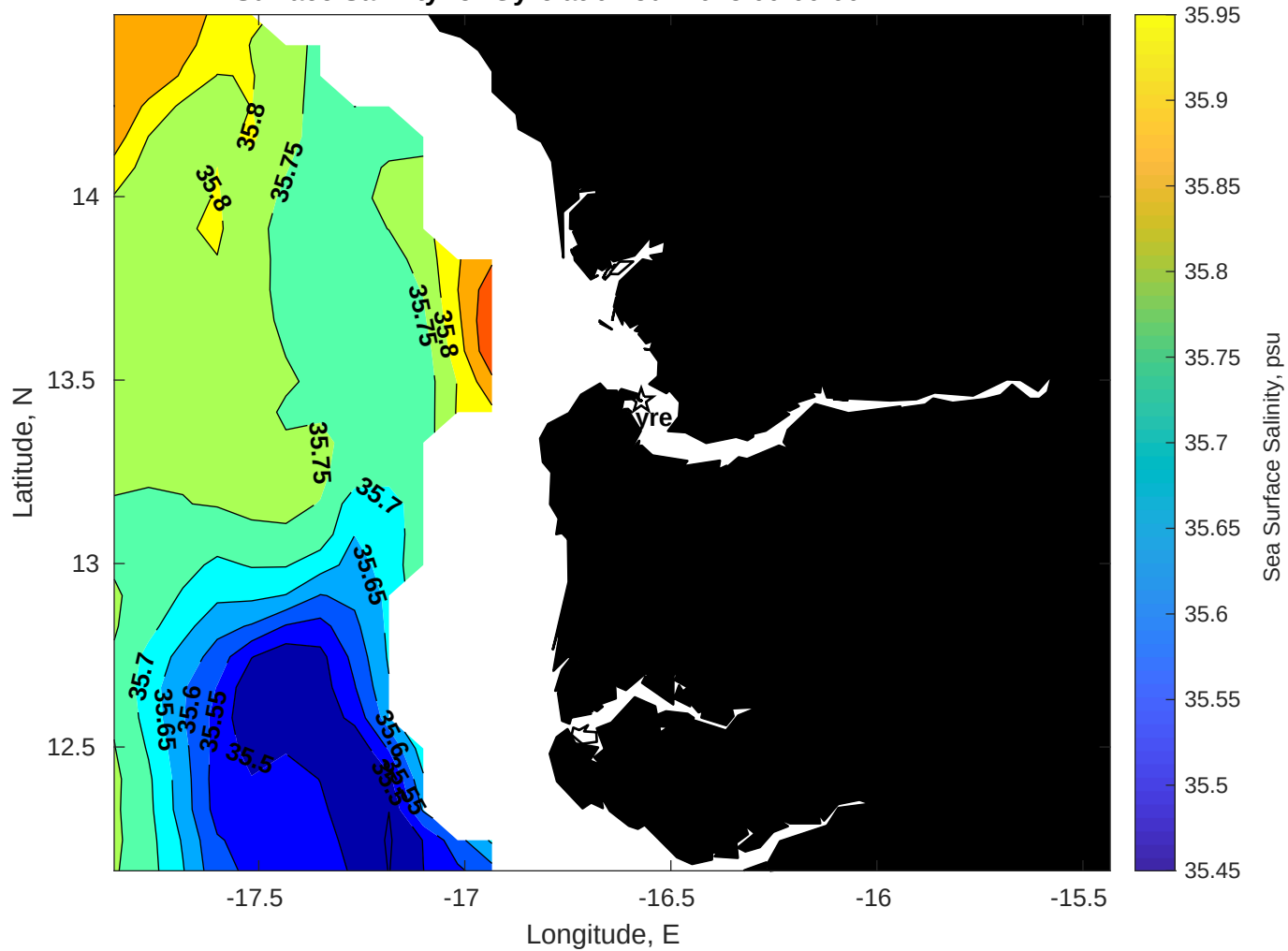
Surface Salinity for Gyre at 01-Jul-2025 00:00:00
