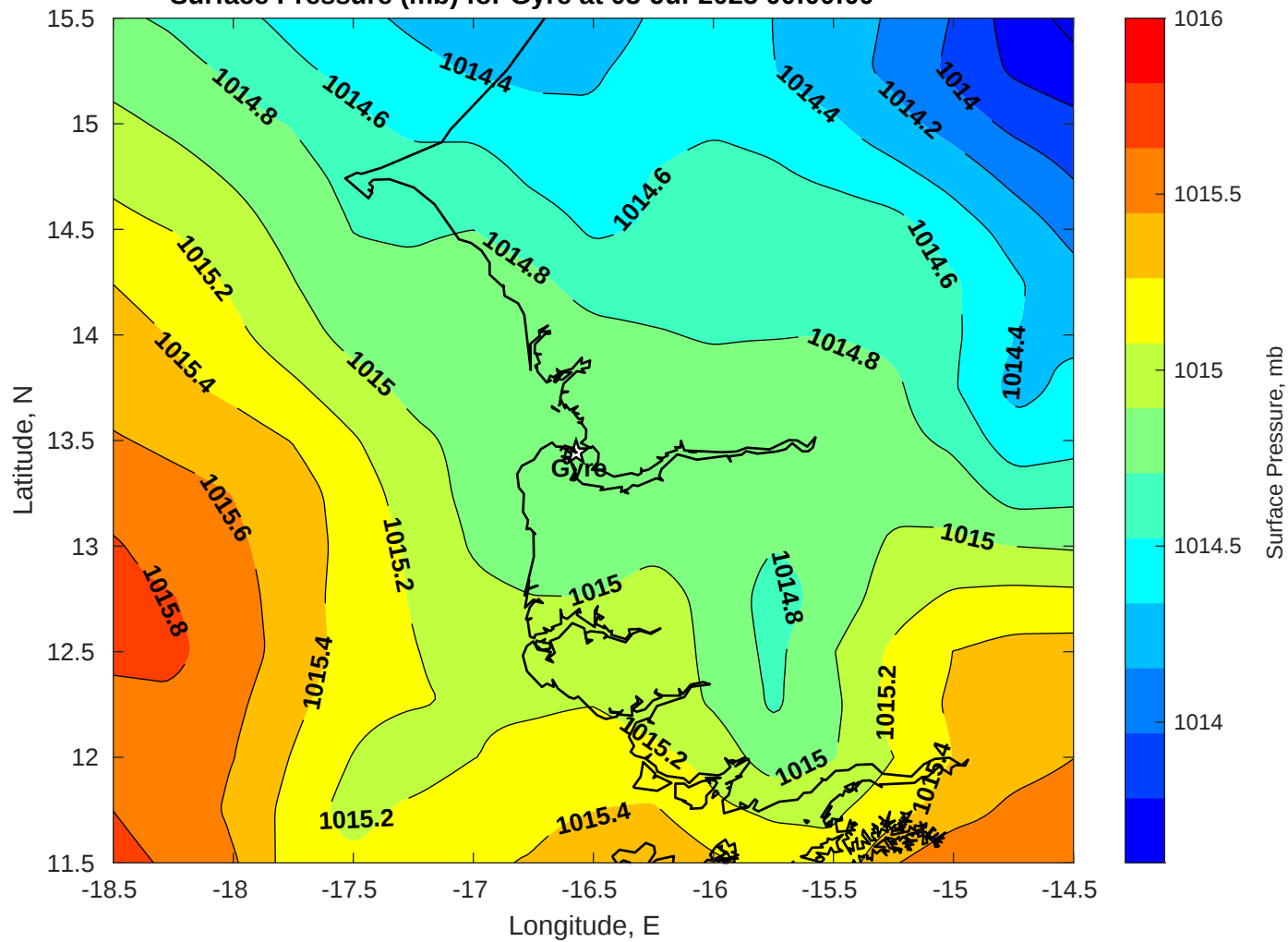
Surface Pressure (mb) for Gyre at 03-Jul-2025 00:00:00
