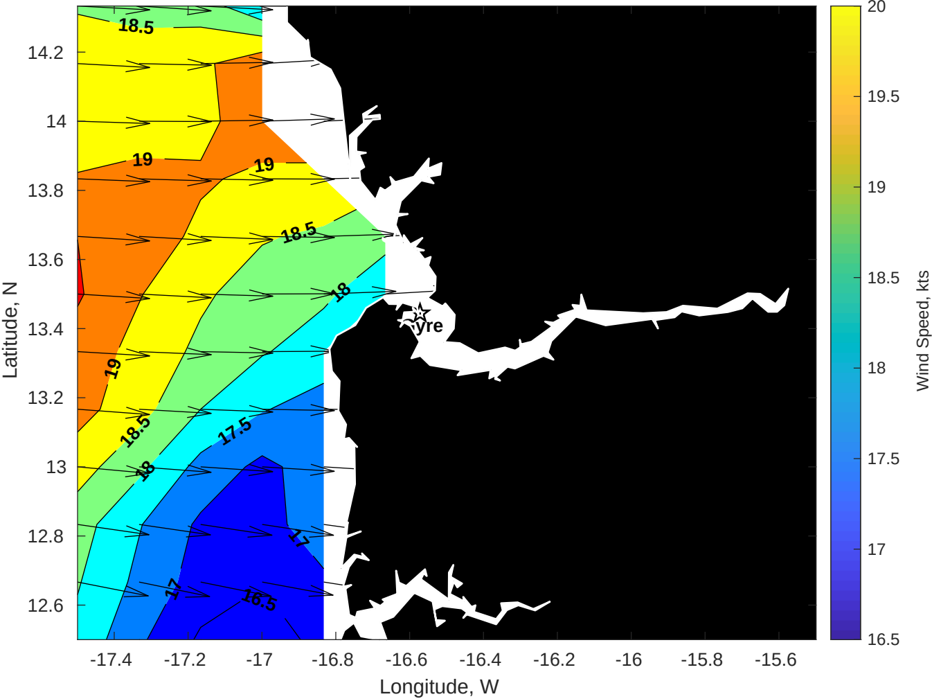
Winds (kts) for Gyre at 02-Jul-2025 09:00:00
