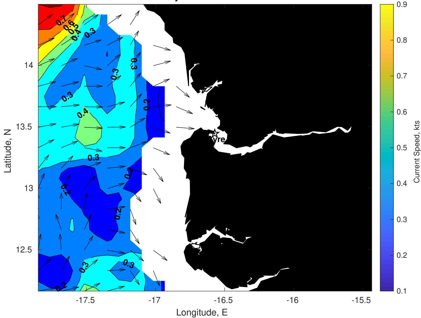
Surface Currents for Gyre at 01-Jul-2025 00:00:00
