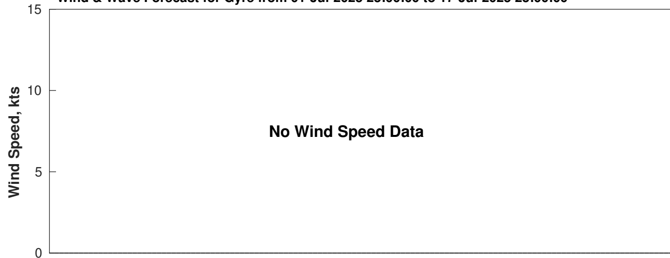
Wind & Wave Forecast for Gyre from 01-Jul-2025 23:00:00 to 17-Jul-2025 23:00:00
