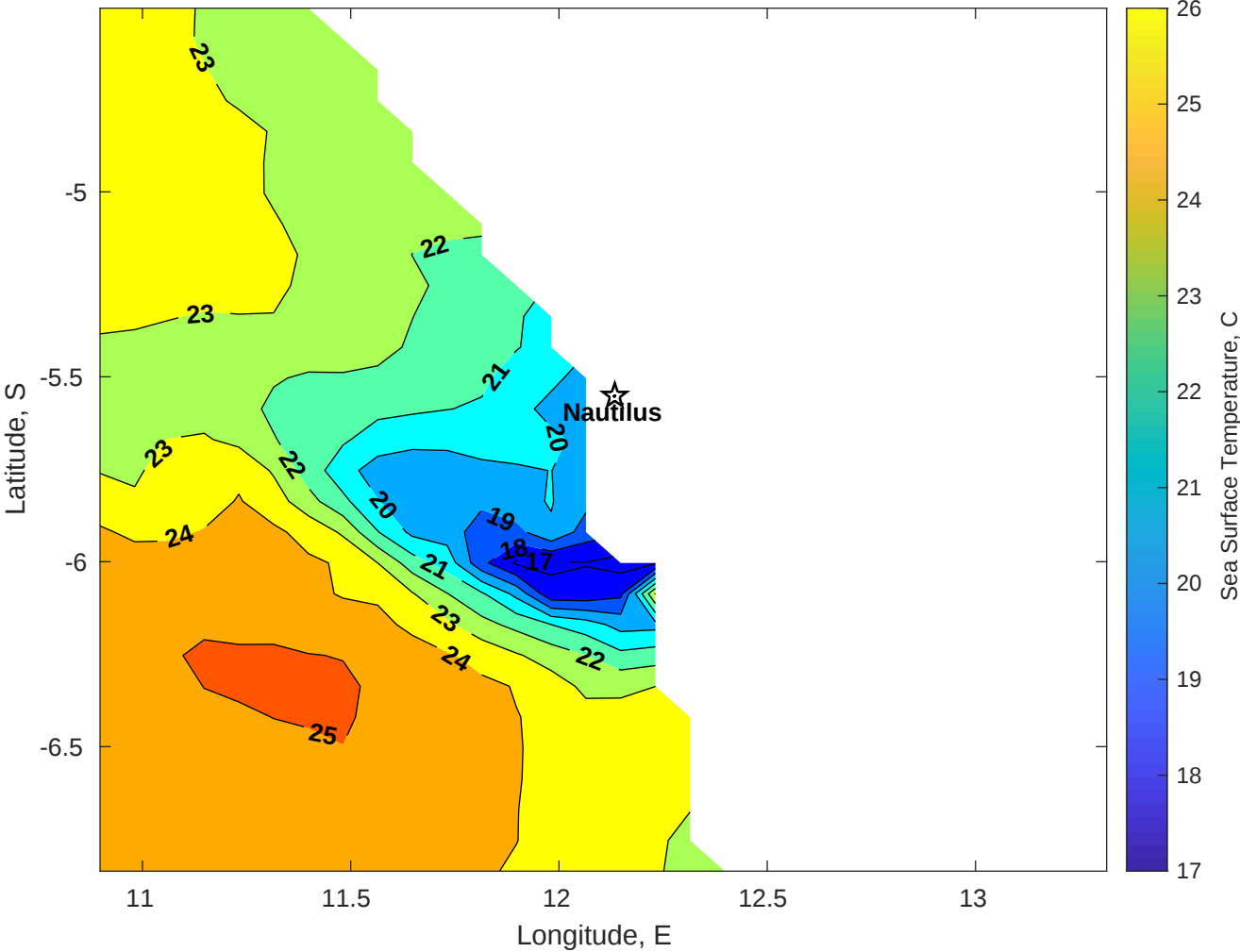
SST for Nautilus at 01-Jul-2025 00:00:00
