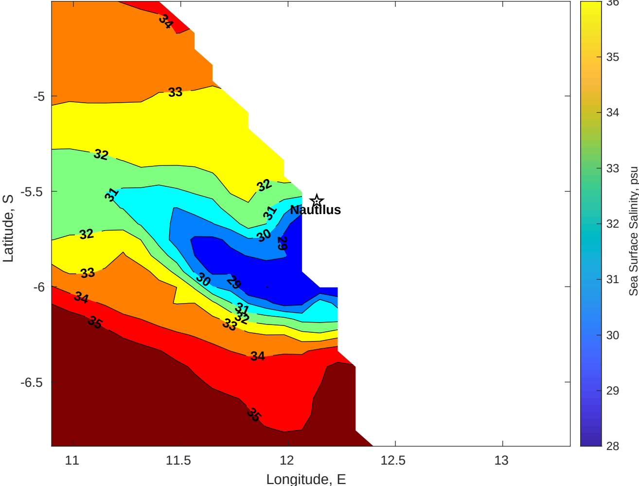
Surface Salinity for Nautilus at 01-Jul-2025 00:00:00
