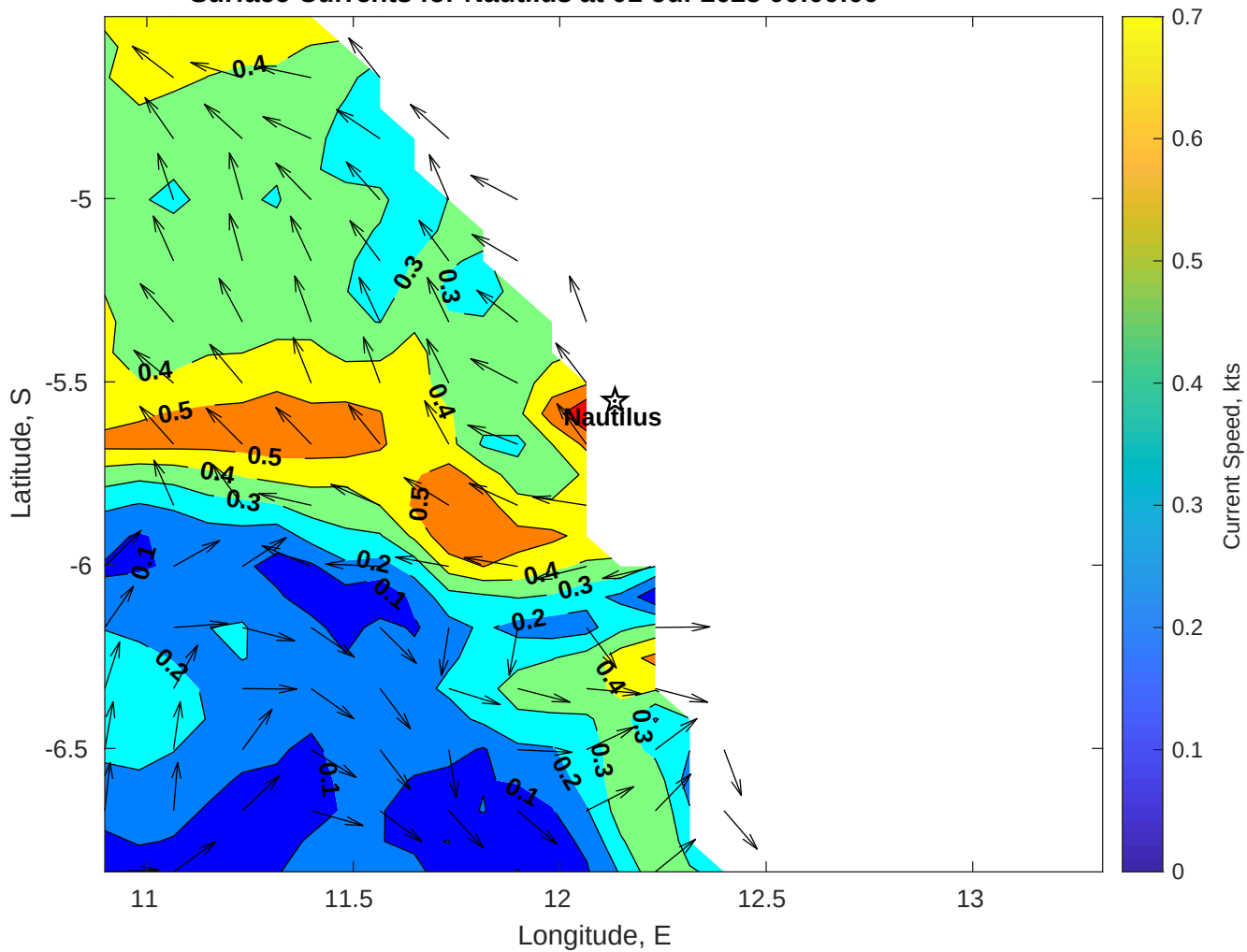
Surface Currents for Nautilus at 01-Jul-2025 00:00:00
