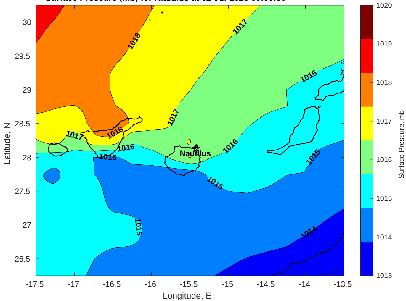
Surface Pressure (mb) for Nautilus at 02-Jul-2025 00:00:00
