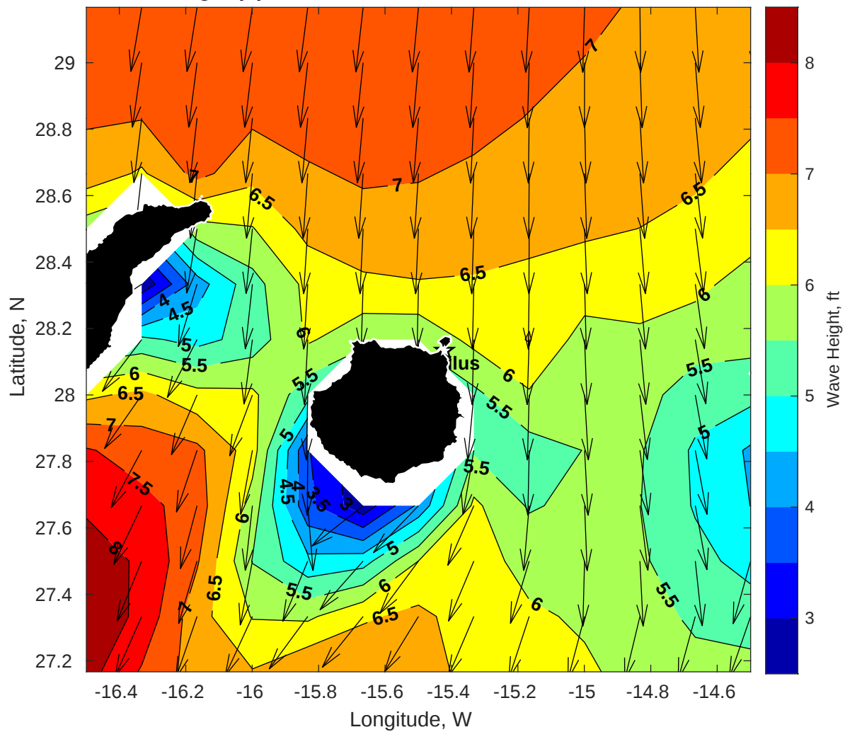
Wave Height (ft) for Nautilus at 02-Jul-2025 09:00:00
