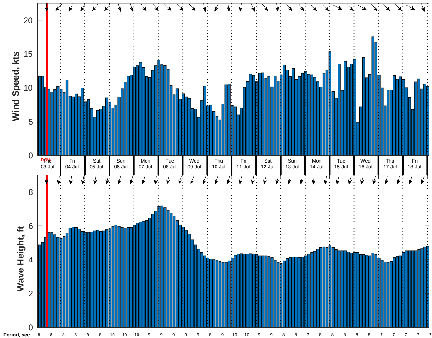
Wind & Wave Forecast for Nautilus from 02-Jul-2025 02:00:00 to 18-Jul-2025 02:00:00
