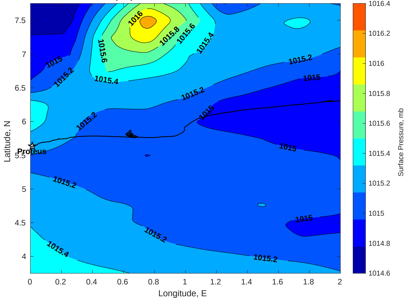
Surface Pressure (mb) for Proteus at 19-Jun-2025 00:00:00
