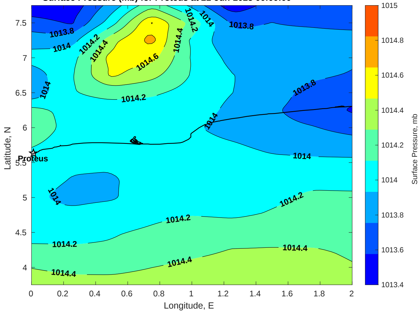
Surface Pressure (mb) for Proteus at 21-Jun-2025 00:00:00
