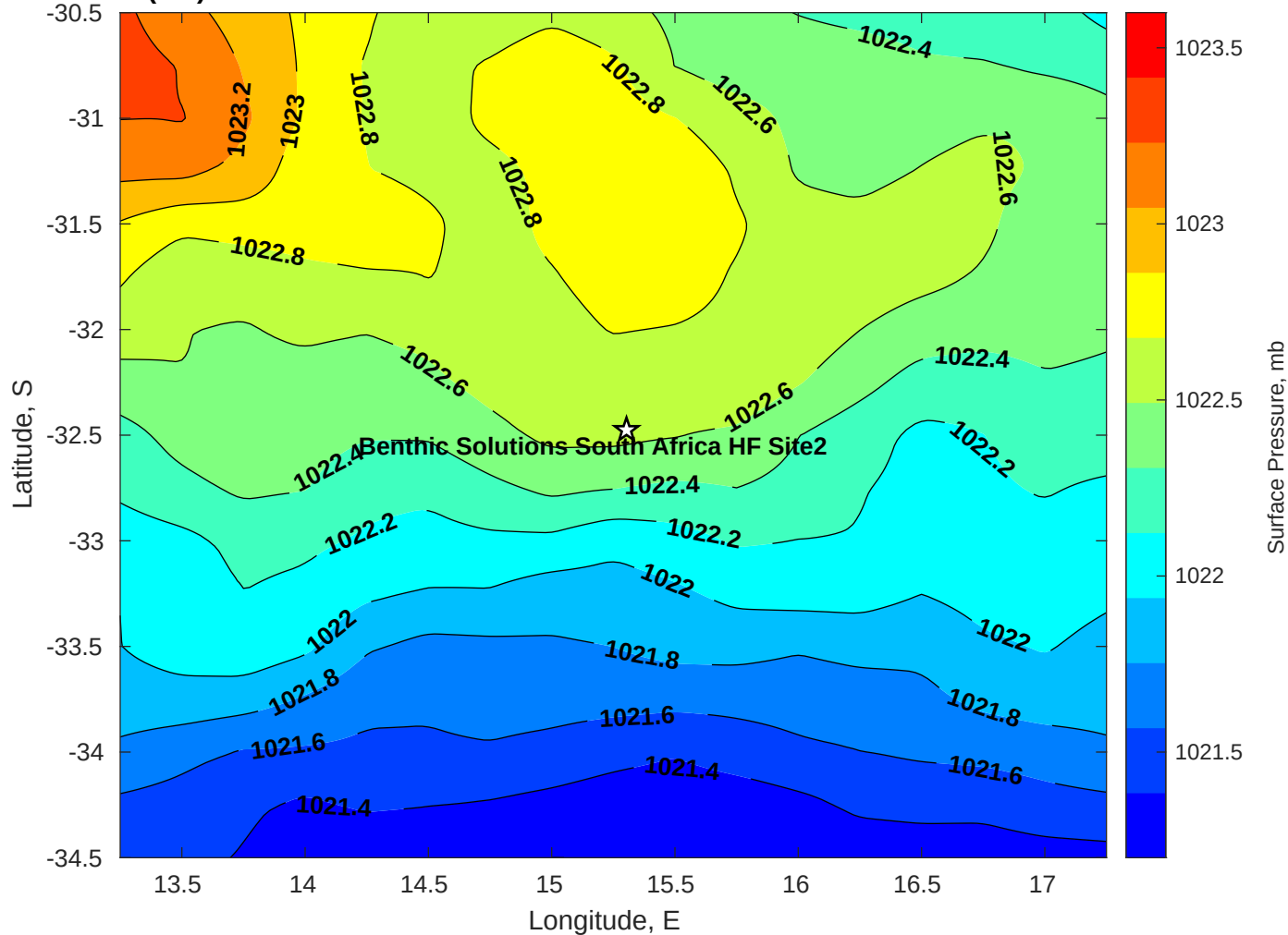
Surface Pressure (mb) for Benthic Solutions South Africa HF Site2 at 19-Jun-2025 00:00:00
