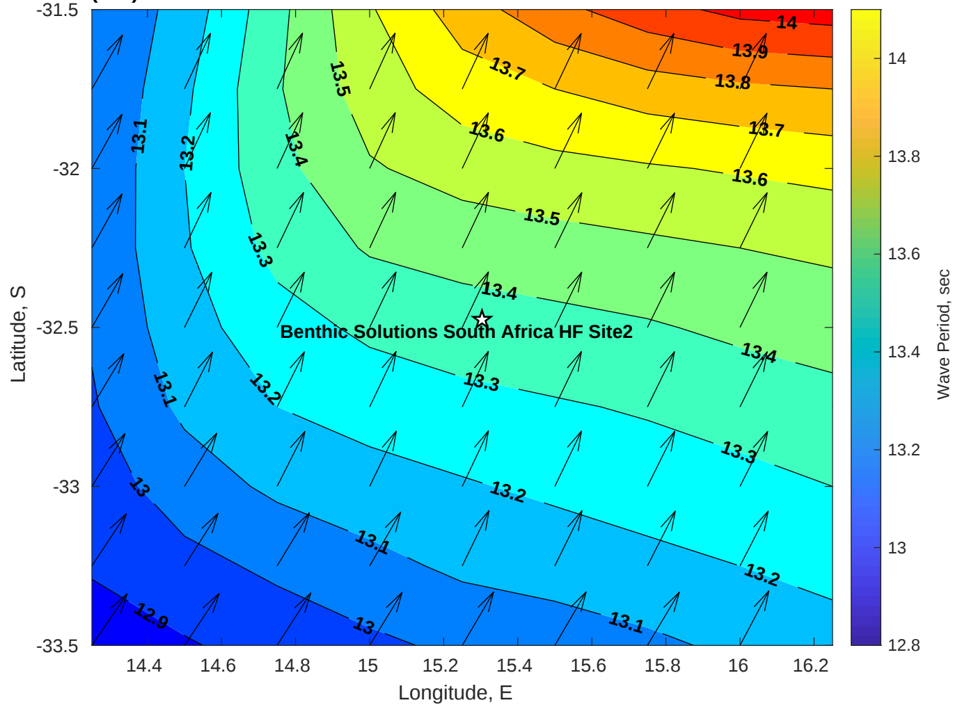
Wave Period (sec) for Benthic Solutions South Africa HF Site2 at 19-Jun-2025 09:00:00
