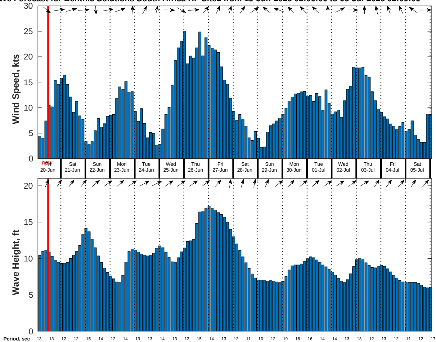
Wind & Wave Forecast for Benthic Solutions South Africa HF Site2 from 19-Jun-2025 02:00:00 to 05-Jul-2025 02:00:00
