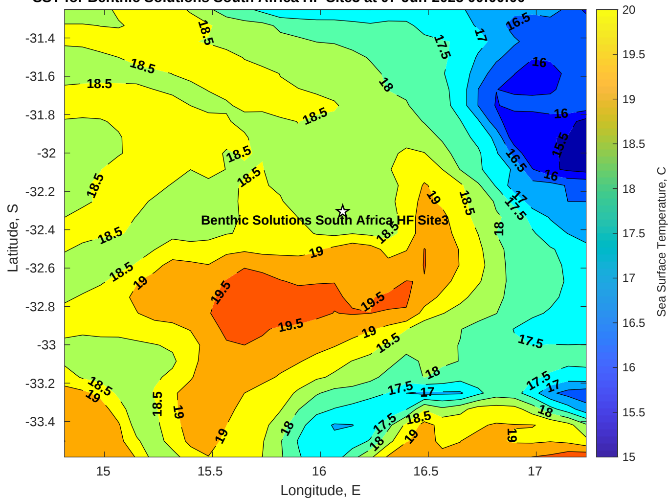
SST for Benthic Solutions South Africa HF Site3 at 07-Jun-2025 00:00:00
