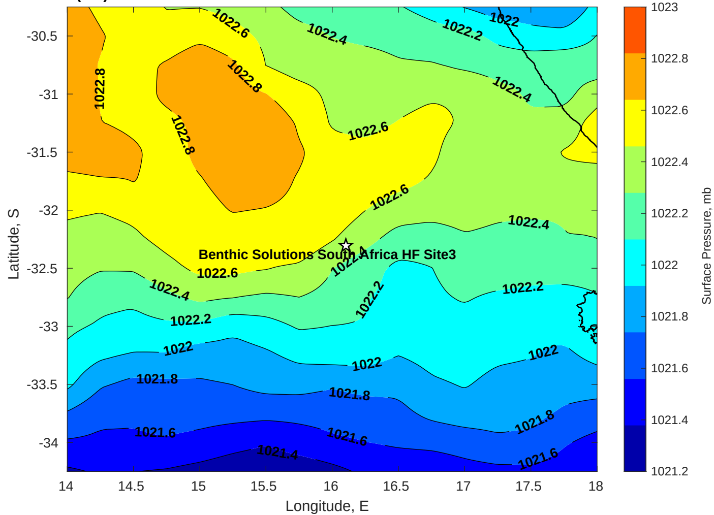
Surface Pressure (mb) for Benthic Solutions South Africa HF Site3 at 19-Jun-2025 00:00:00
