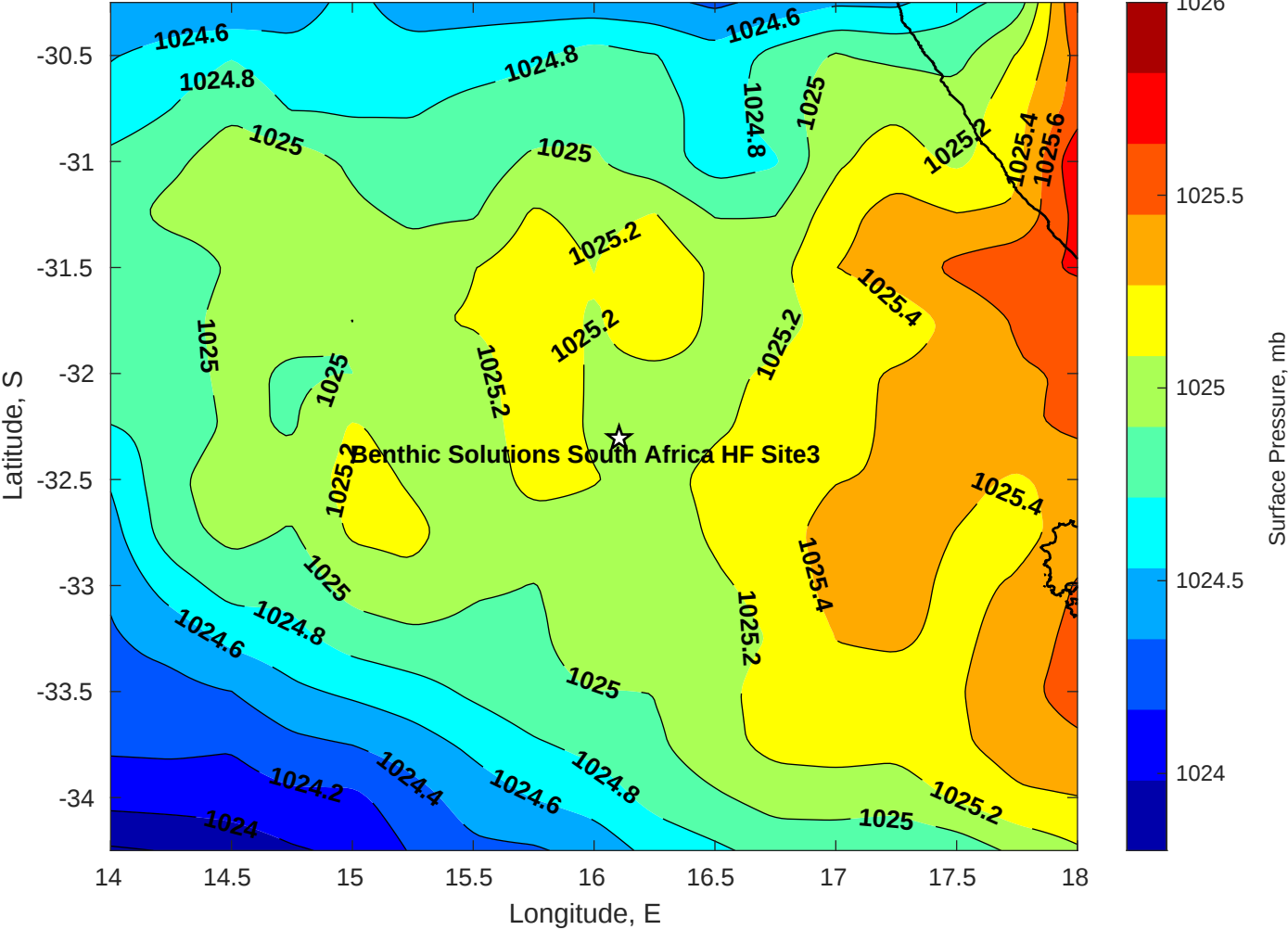
Surface Pressure (mb) for Benthic Solutions South Africa HF Site3 at 21-Jun-2025 00:00:00
