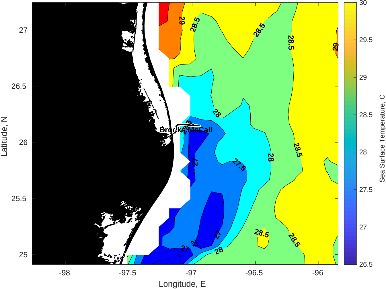
SST for Brooks McCall at 02-Jul-2025 00:00:00
