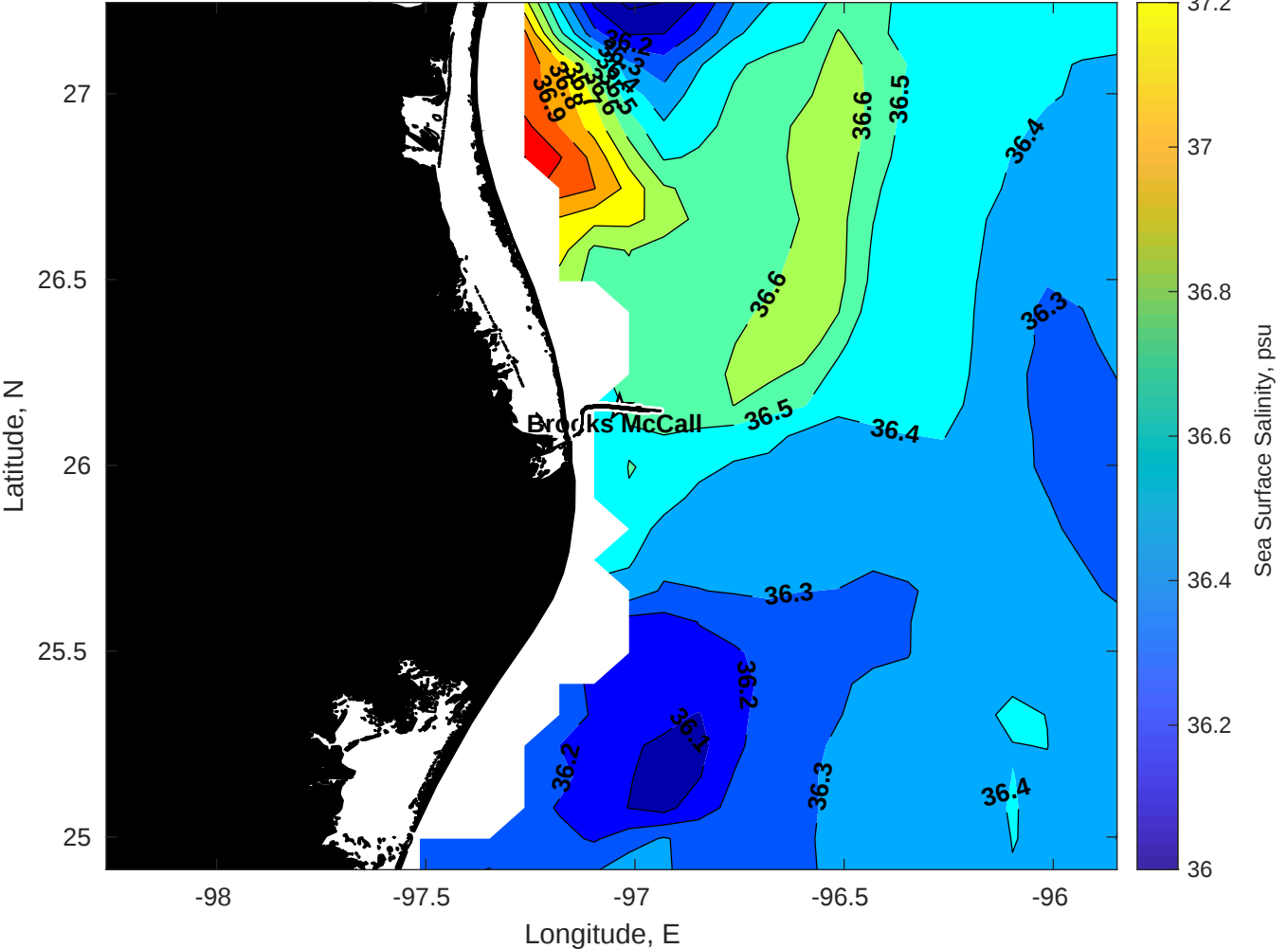
Surface Salinity for Brooks McCall at 02-Jul-2025 00:00:00
