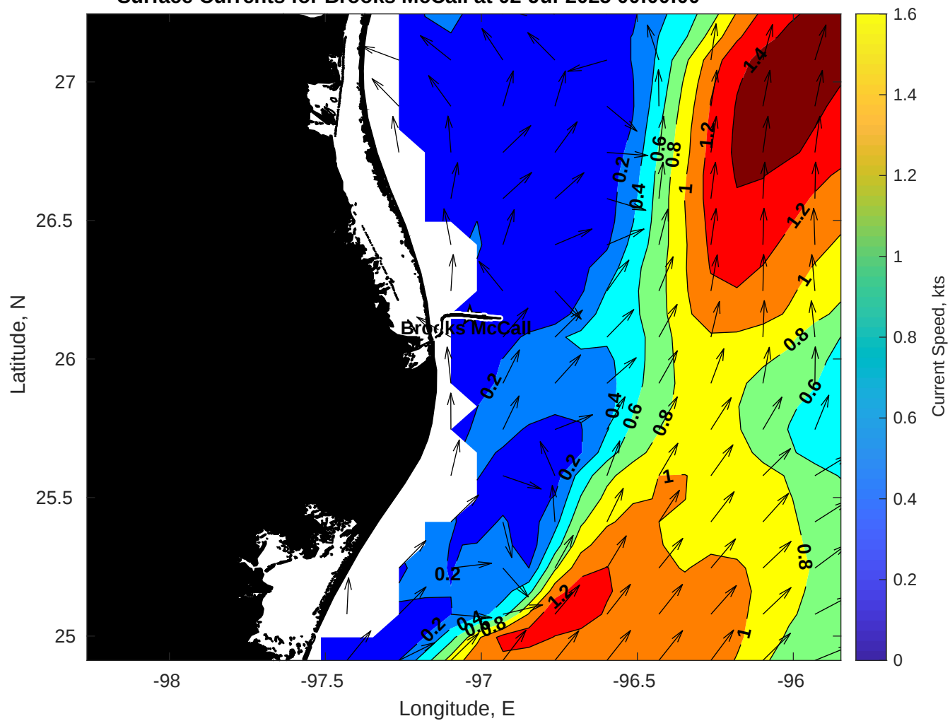
Surface Currents for Brooks McCall at 02-Jul-2025 00:00:00
