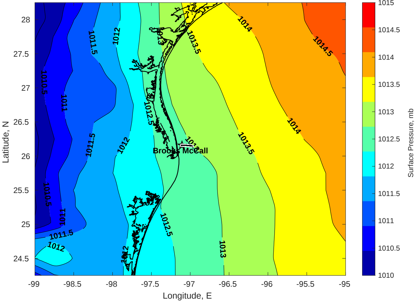
Surface Pressure (mb) for Brooks McCall at 04-Jul-2025 00:00:00
