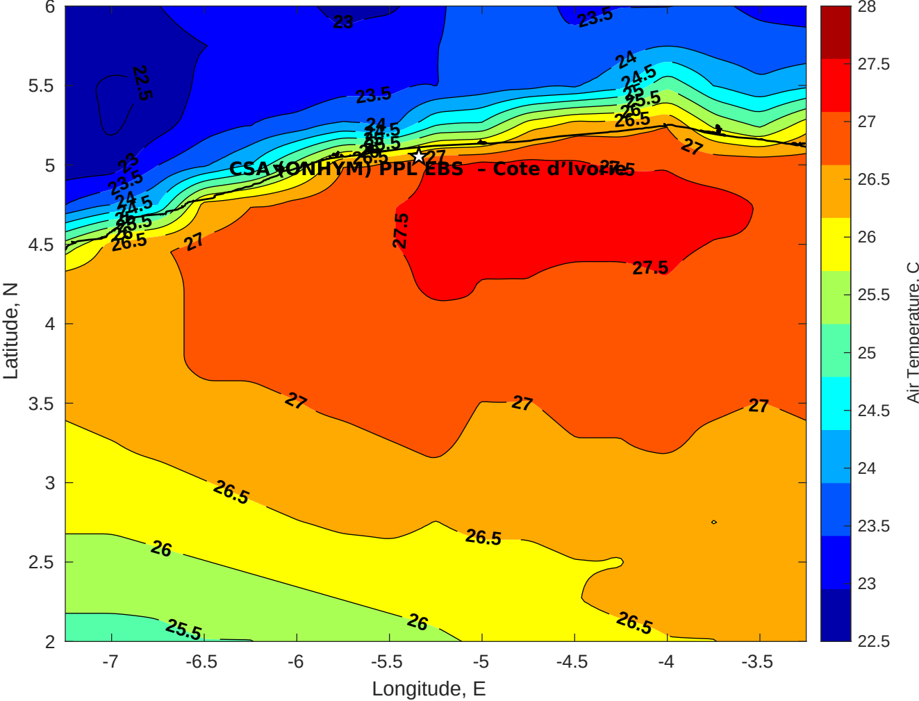
Air Temperature (C) for CSA (ONHYM) PPL EBS - Cote d'Ivoire at 19-Jun-2025
