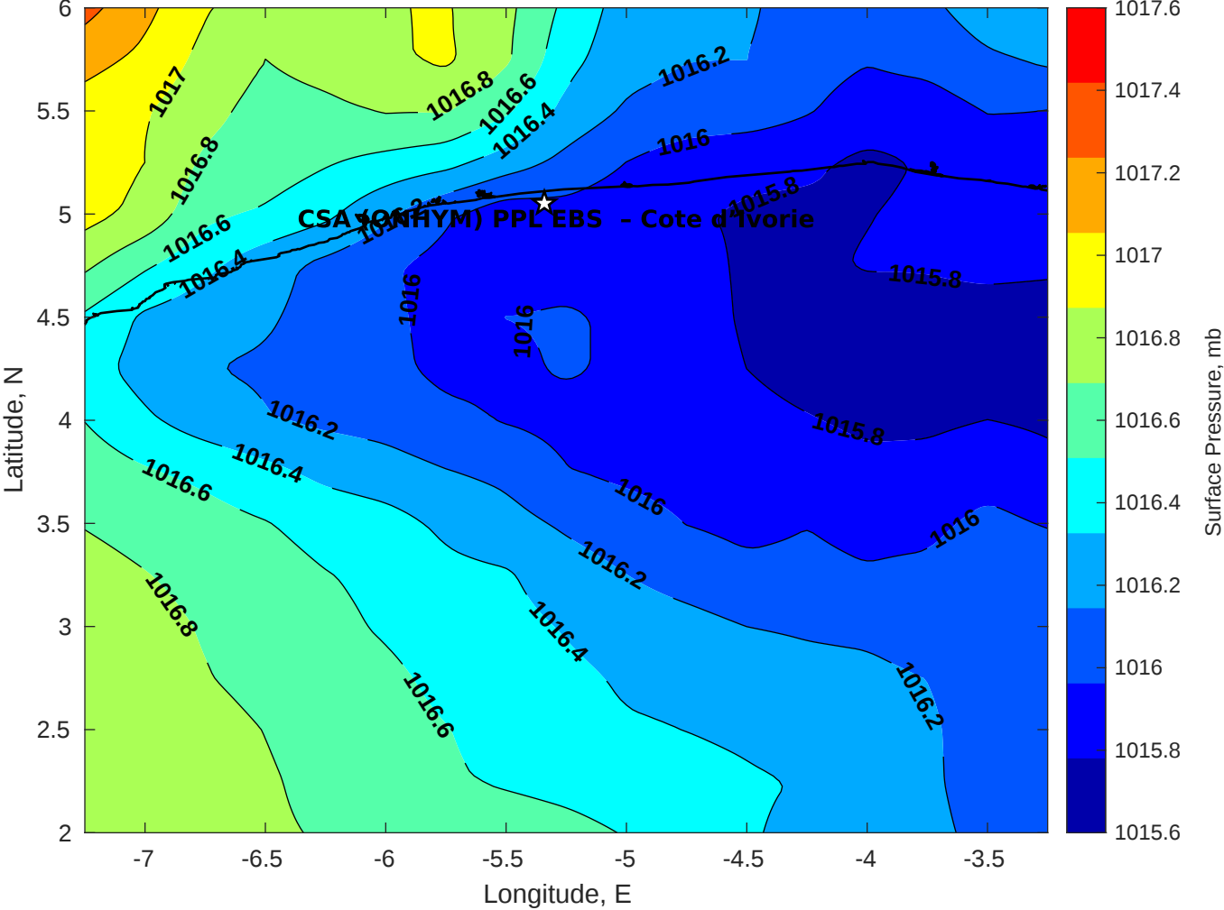
Surface Pressure (mb) for CSA (ONHYM) PPL EBS - Cote d'Ivoire at 19-Jun-2025 00:00:00
