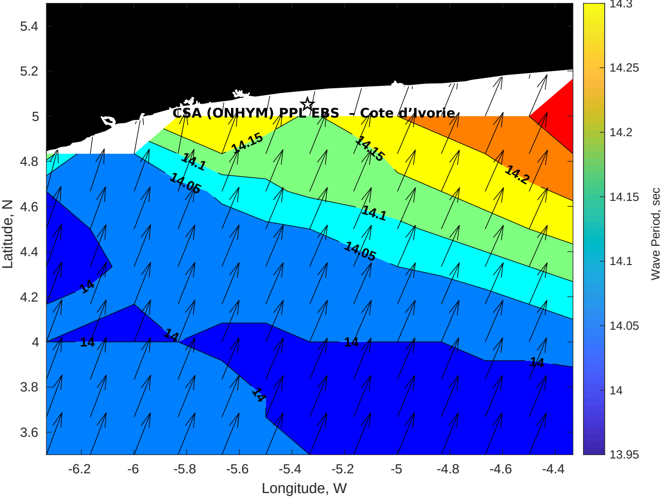
Wave Period (sec) for CSA (ONHYM) PPL EBS - Cote d'Ivoire at 19-Jun-2025 09:00:00
