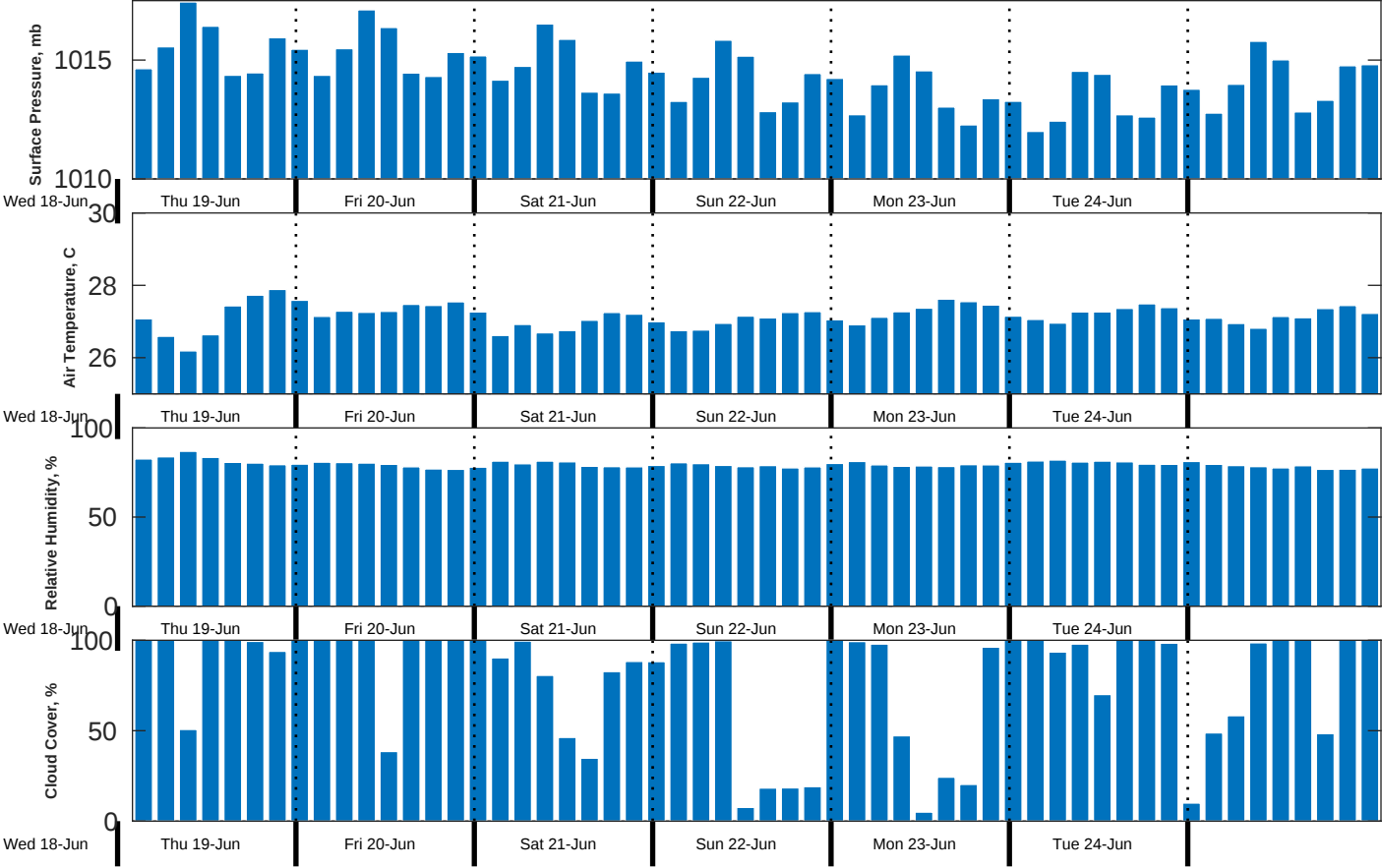
Met Forecast for CSA (ONHYM) PPL EBS - Cote d'Ivoire from 19-Jun-2025 00:00:00 to 26-Jun-2025 00:00:00
